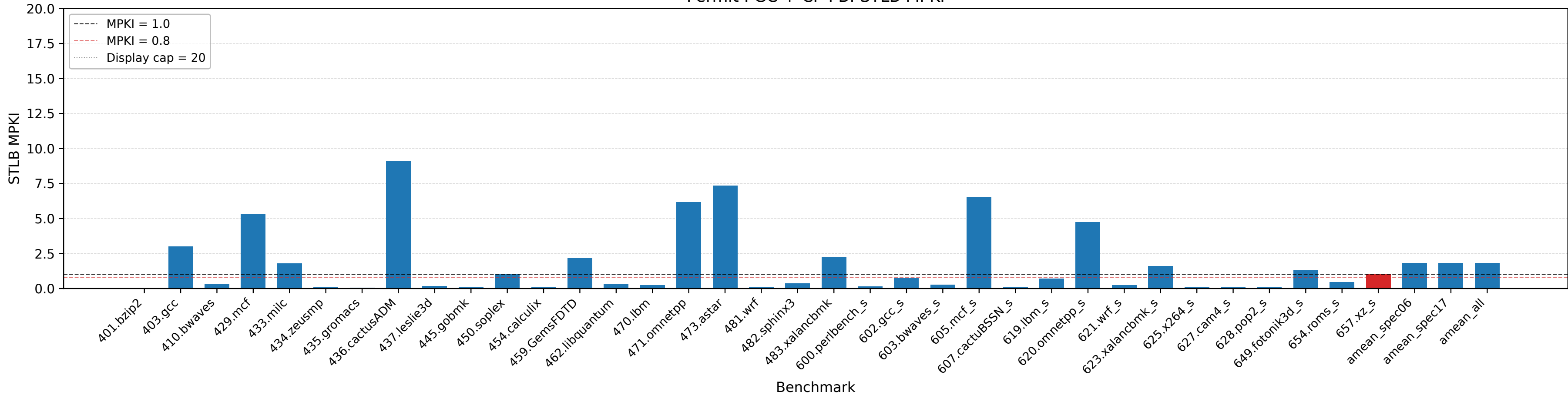
Permit PGC + CP-PB: STLB MPKI
