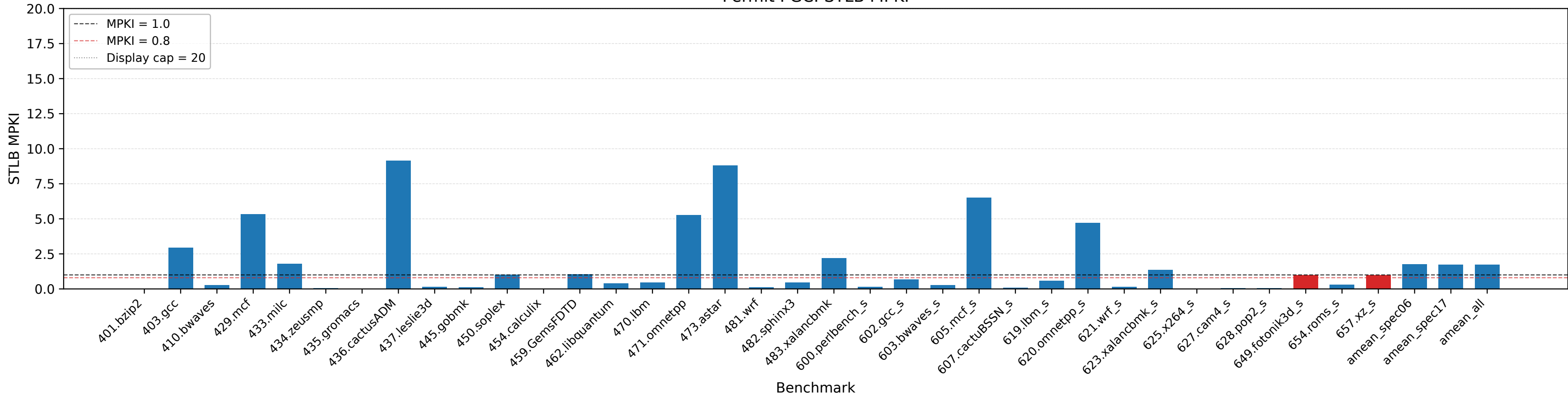
Permit PGC: STLB MPKI
