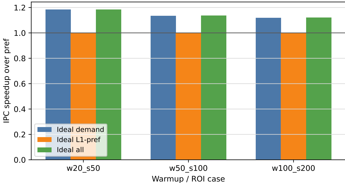
Ideal STLB instruction-count sensitivity
