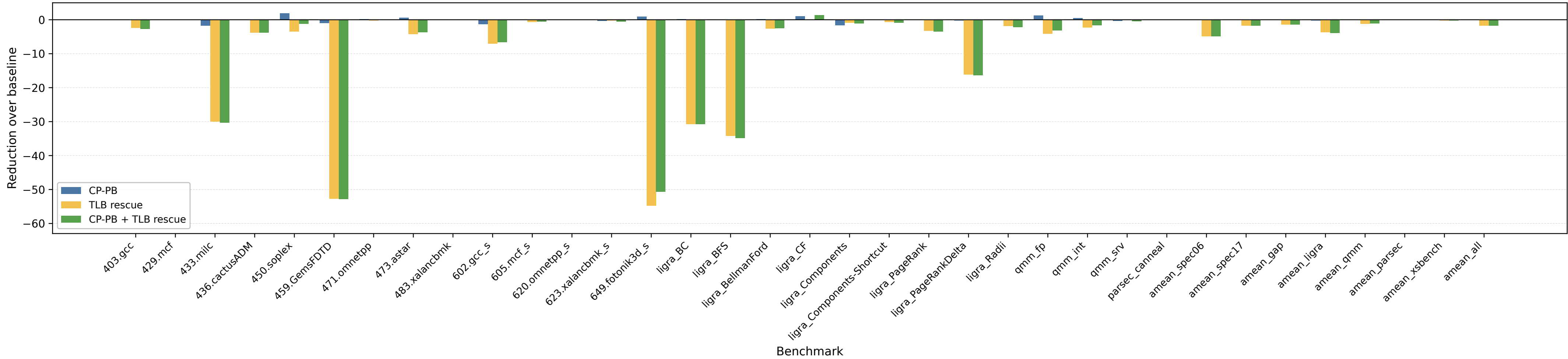
DTLB data demand MPKI reduction over baseline
