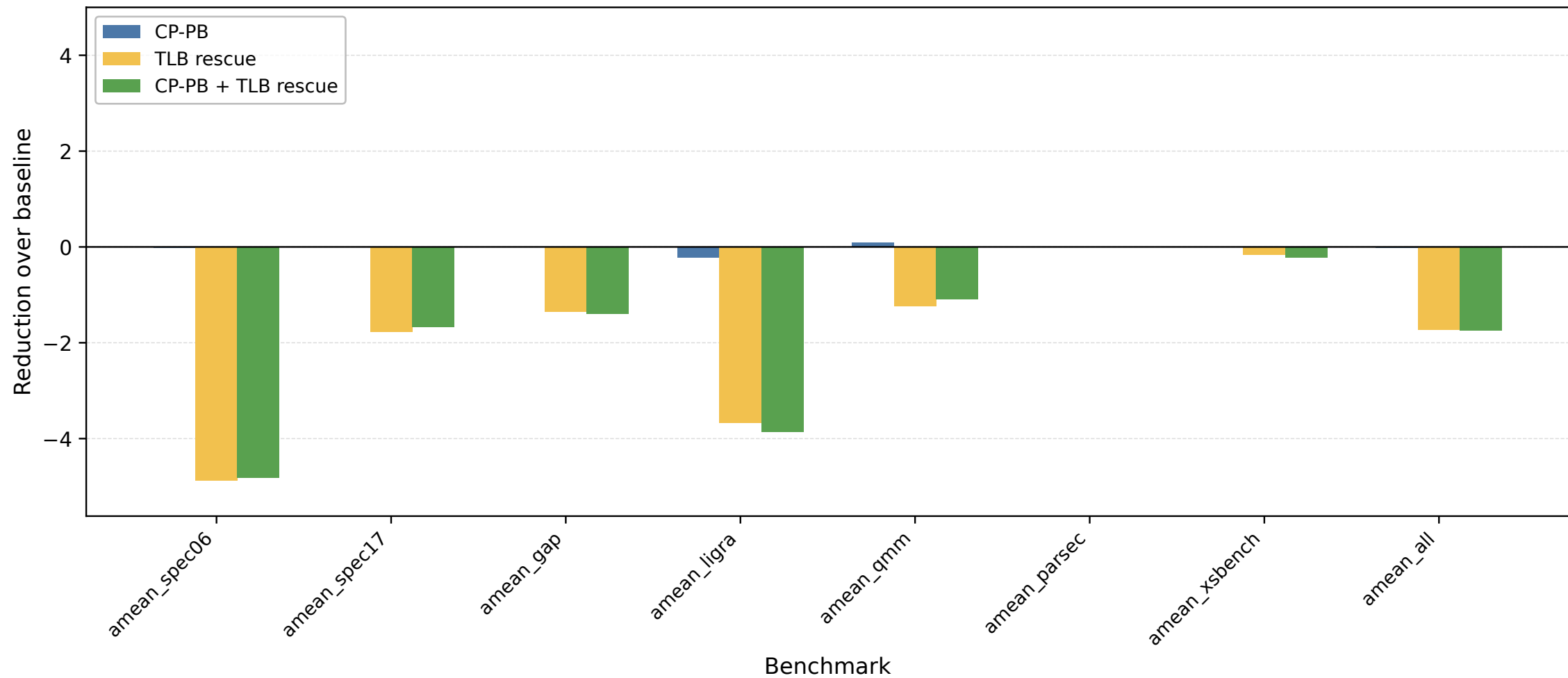
DTLB data demand MPKI reduction over baseline
