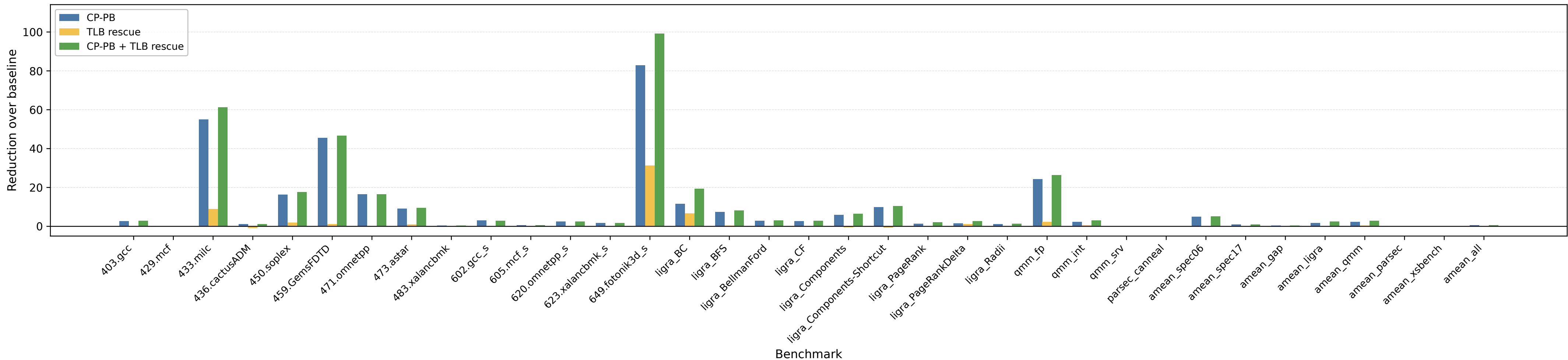
Effective STLB data demand MPKI reduction over baseline
