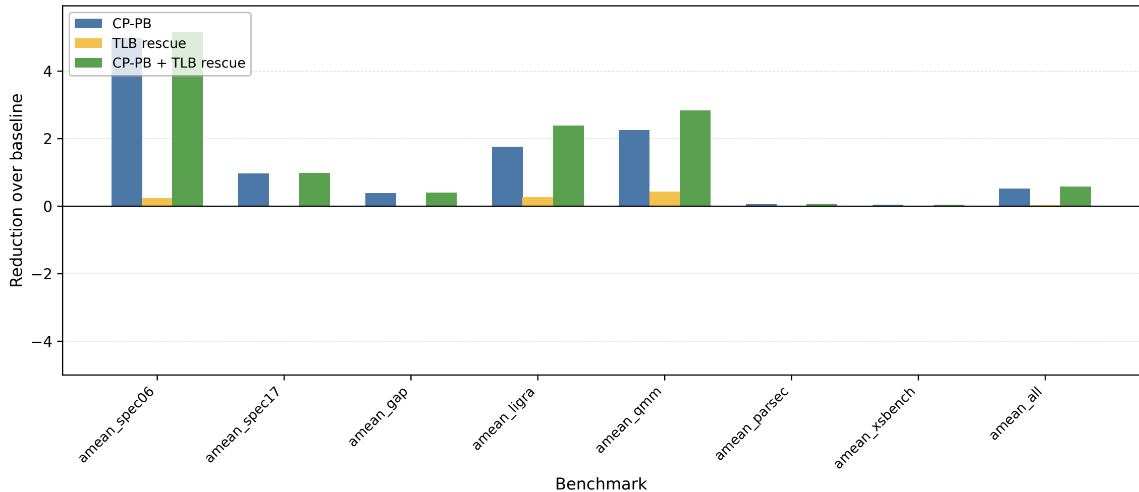
Effective STLB data demand MPKI reduction over baseline
