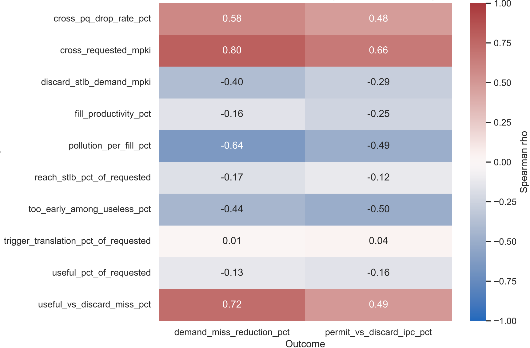
Trace-level monotonic associations (descriptive, not causal)
