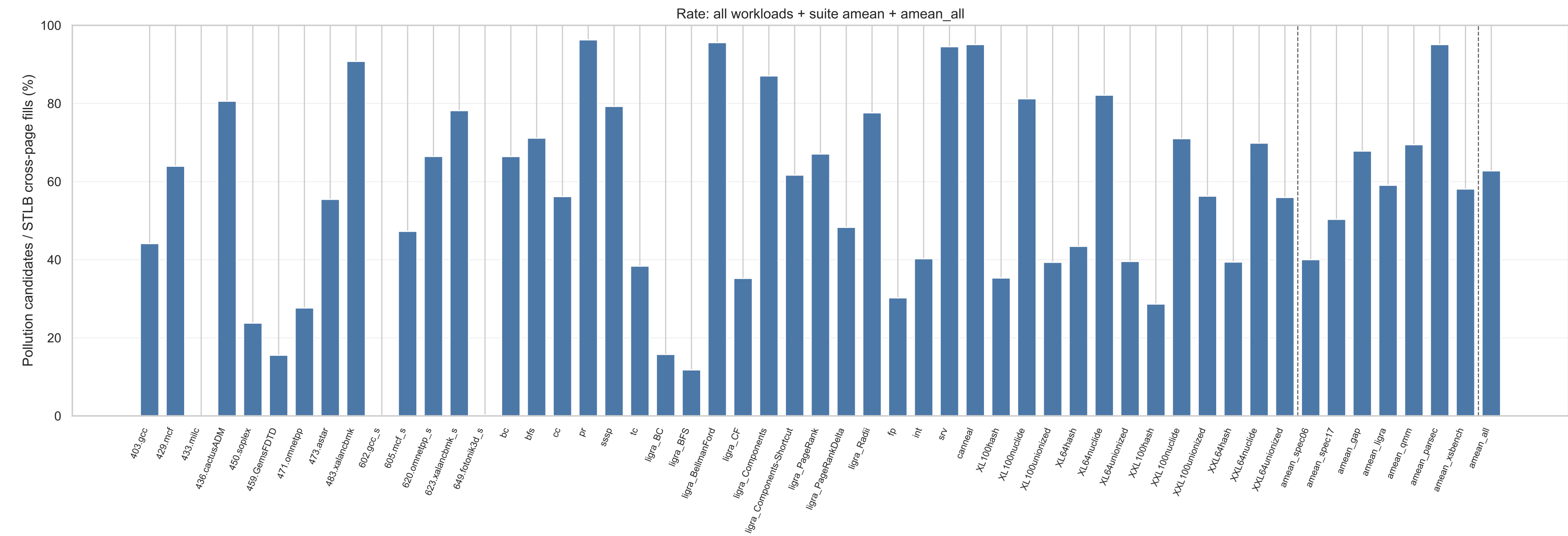
15. vBerti cross-page prefetch pollution candidates at STLB
