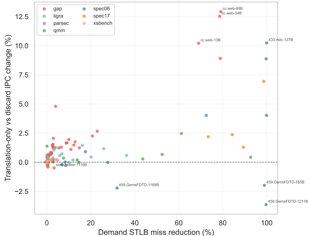
Pure translation mechanism: TLB result vs IPC
