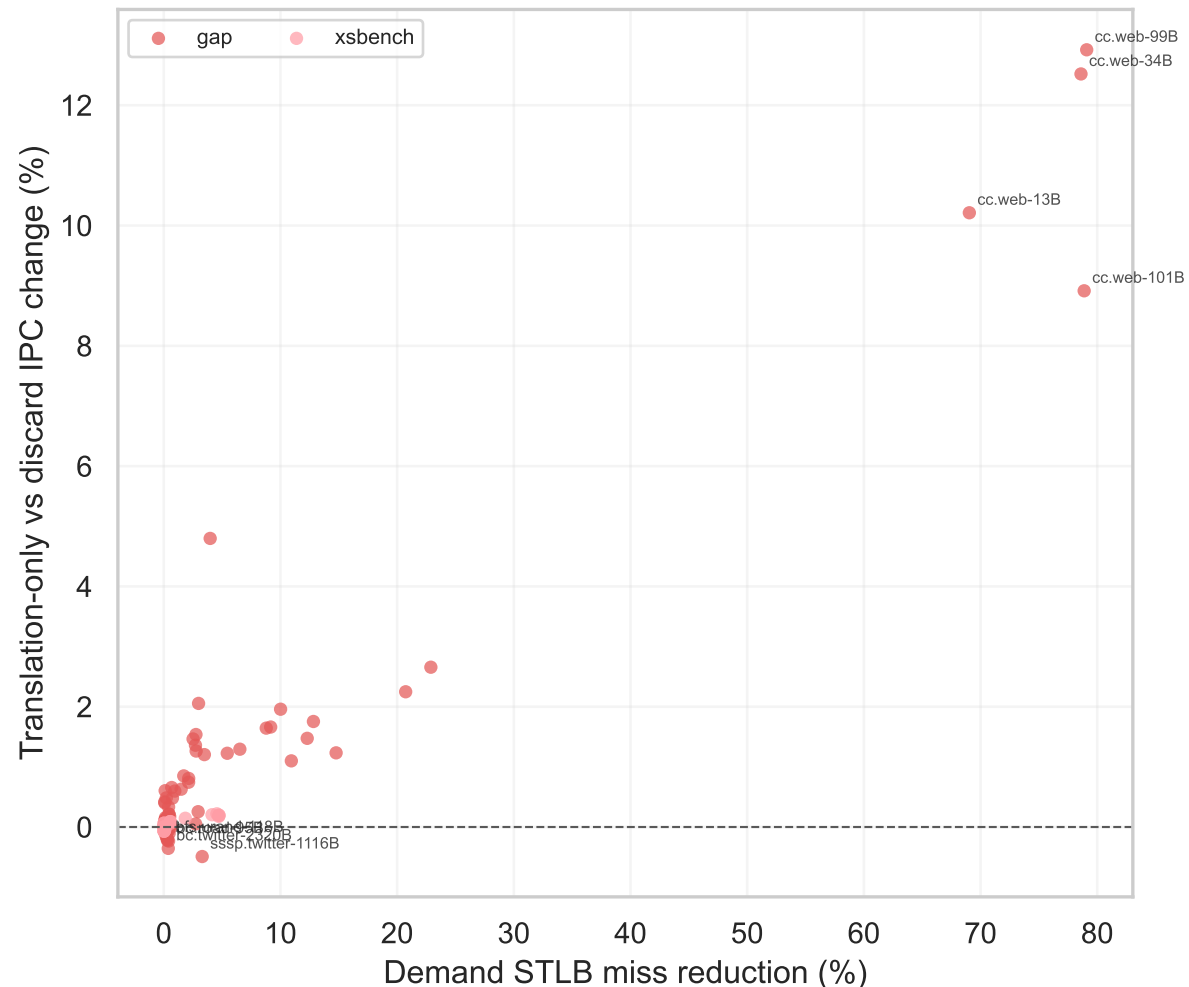
Pure translation mechanism: TLB result vs IPC
