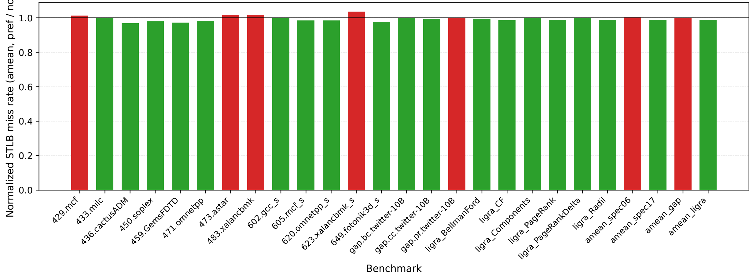
pref vs nopref STLB miss rate amean
