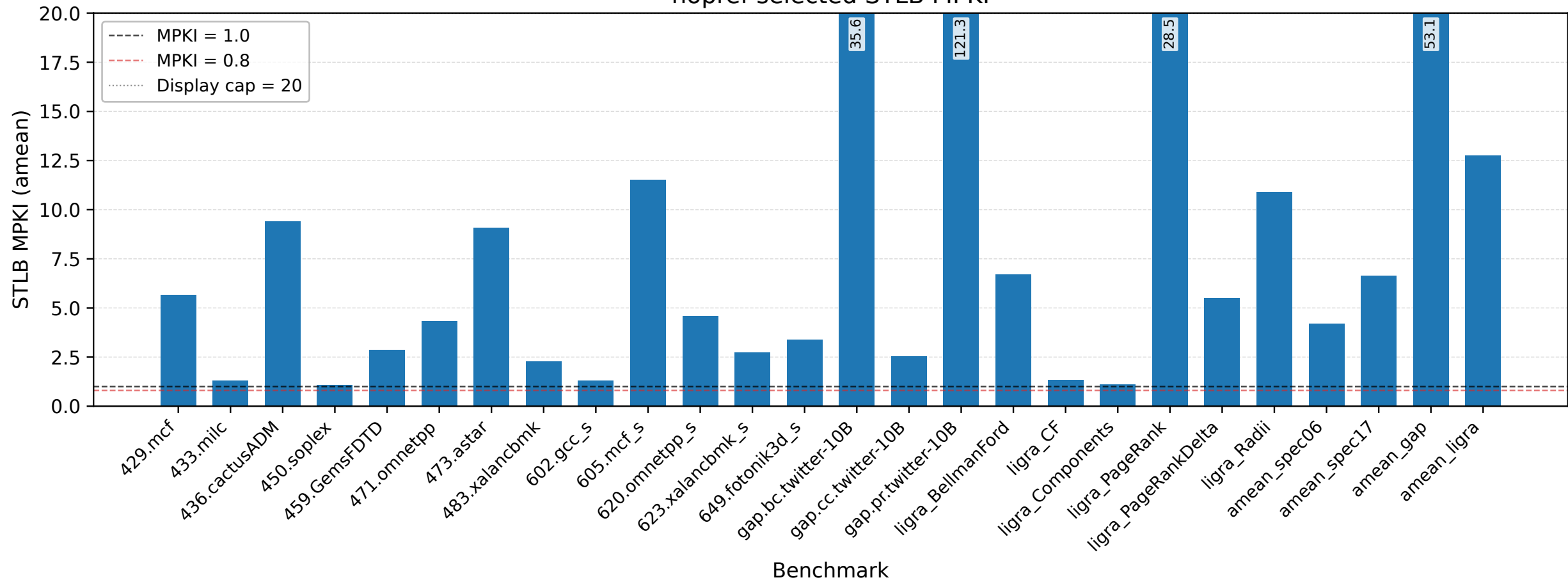
nopref selected STLBP MPKI
