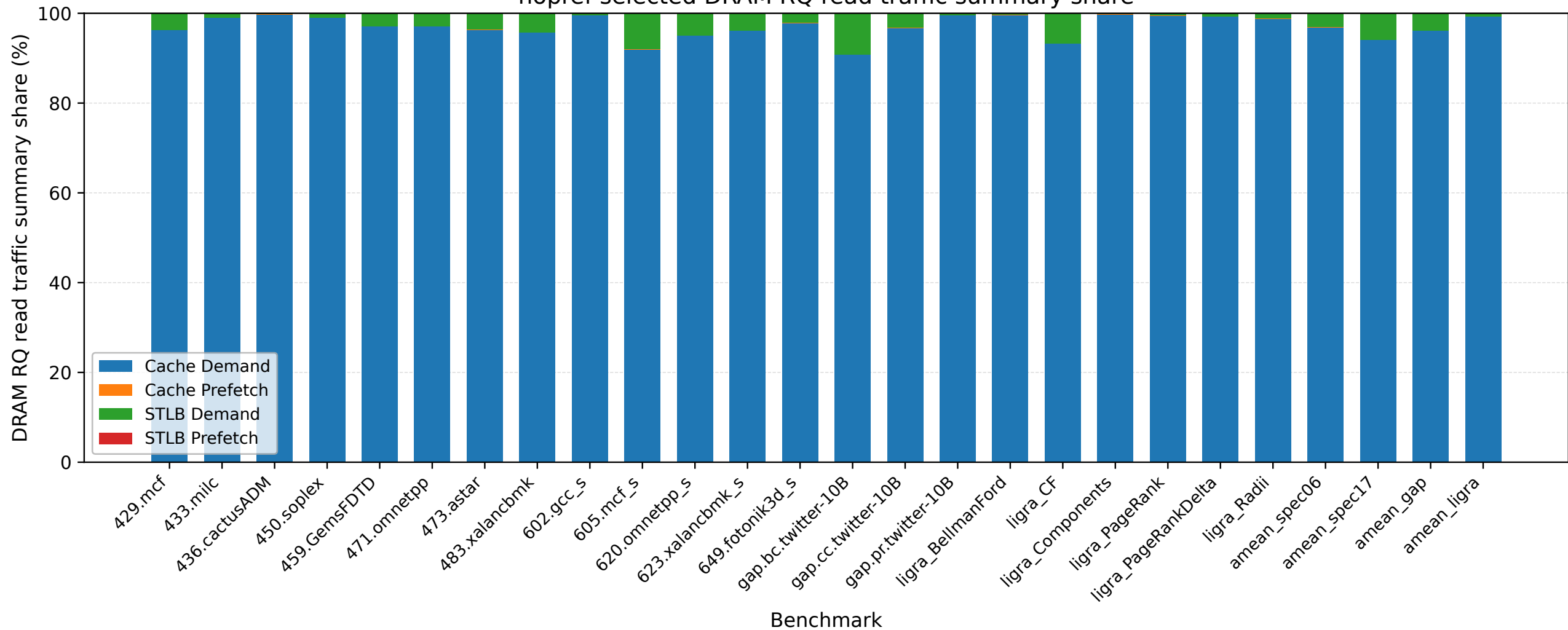
nopref selected DRAM RQ read traffic summary share
