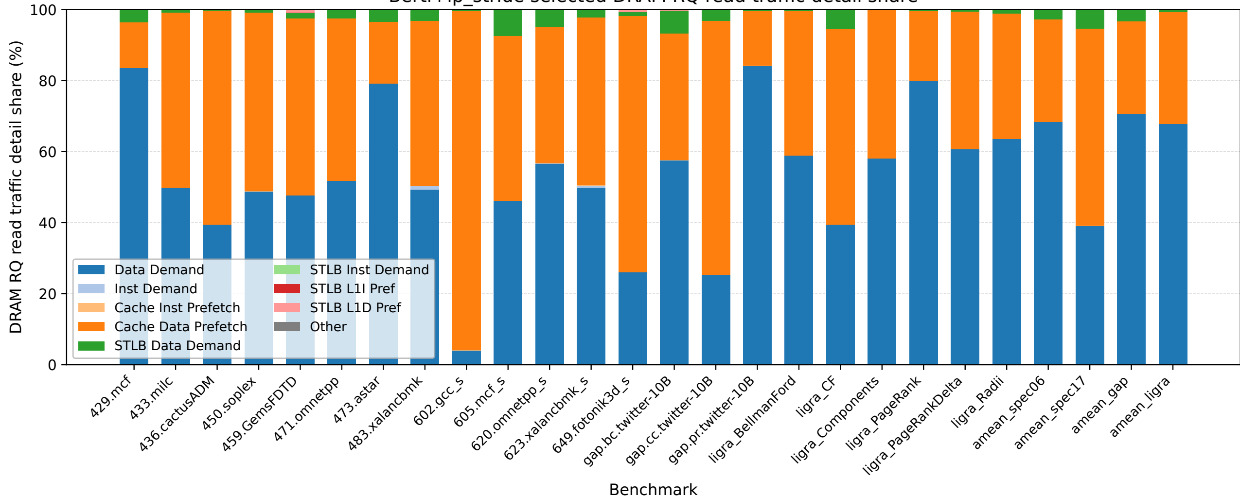
Berti+ip_stride selected DRAM RQ read traffic detail share
