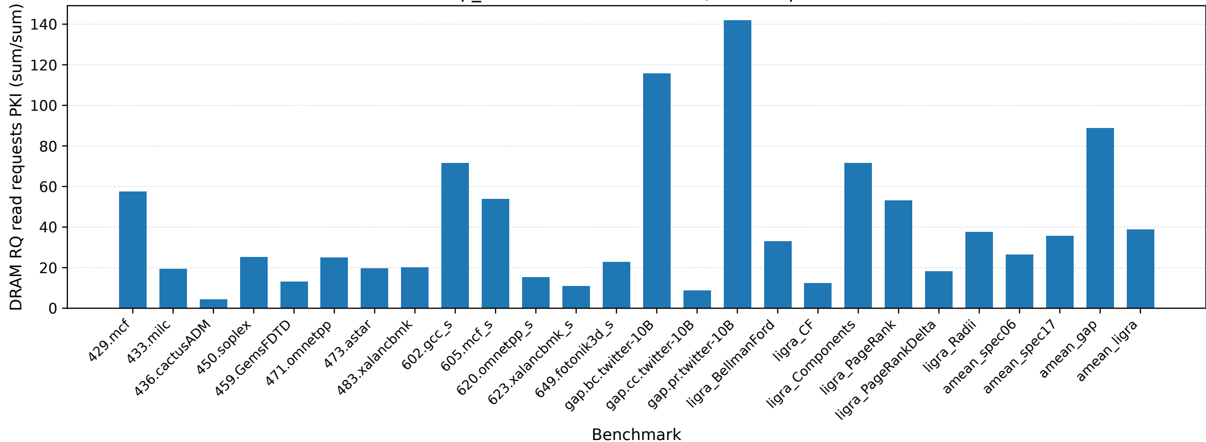
Berti+ip_stride selected DRAM RQ read requests PKI
