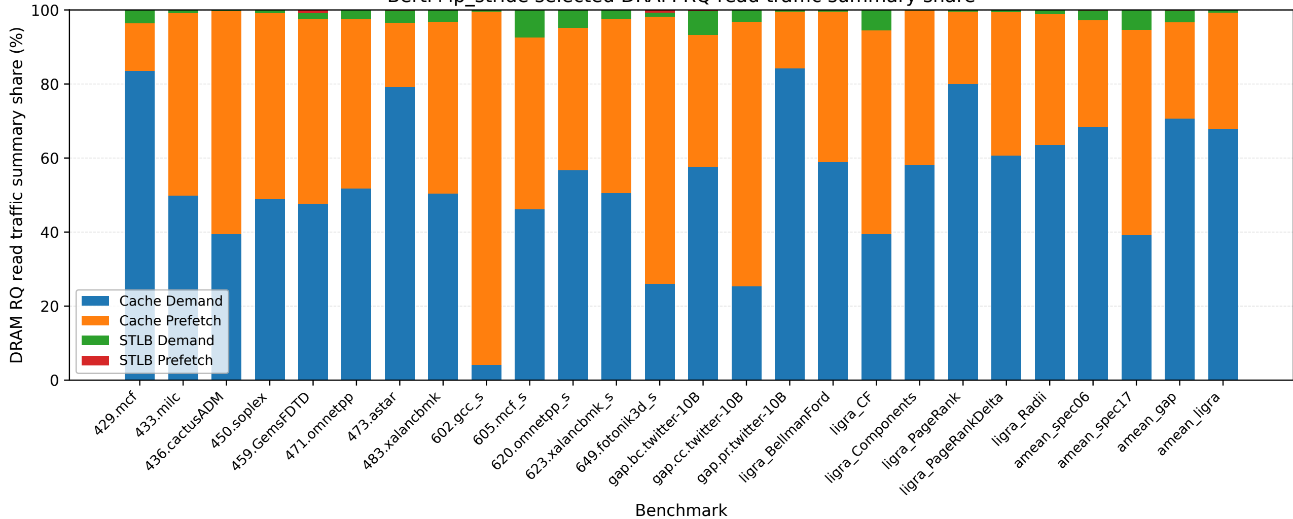
Berti+ip_stride selected DRAM RQ read traffic summary share
