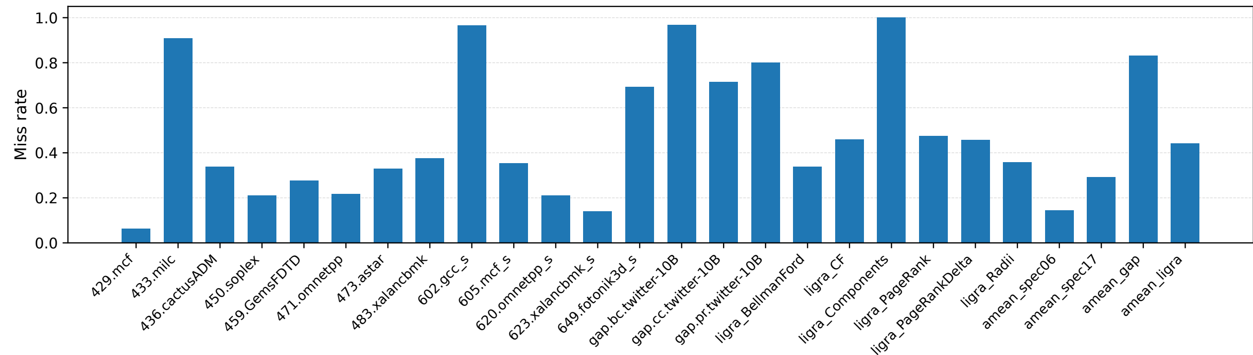
STLB total miss rate
