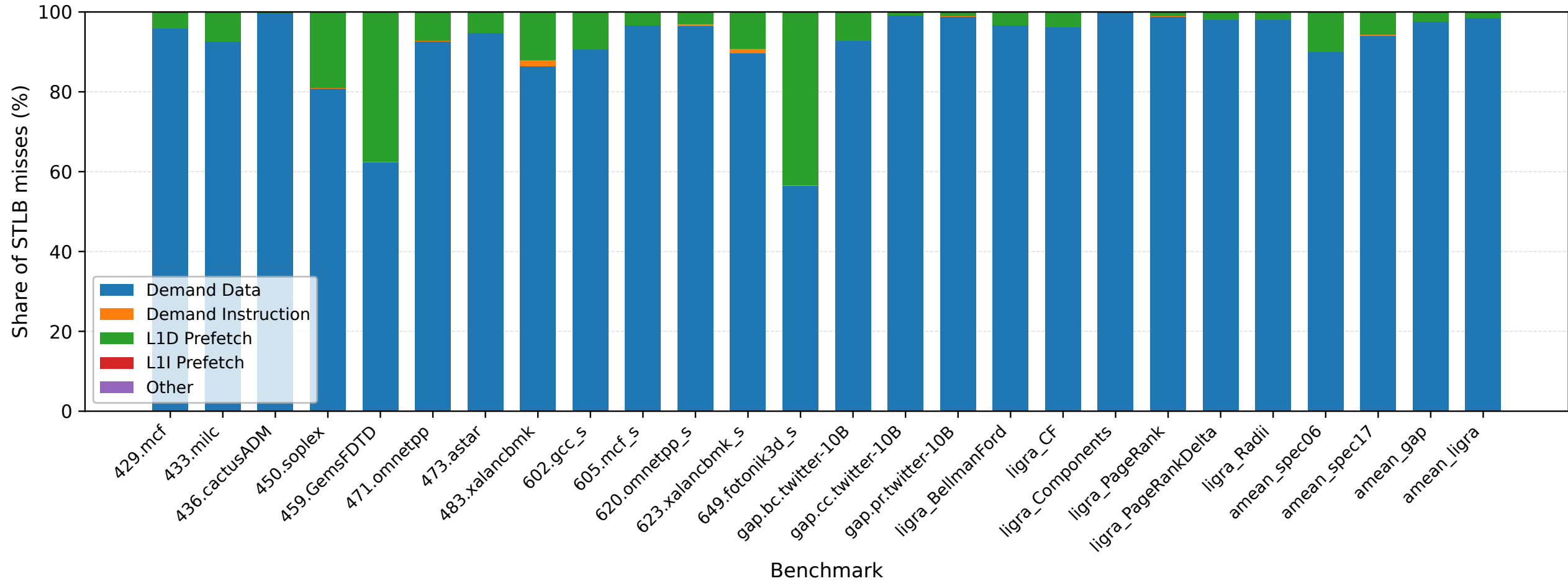
STLB miss-cause share
