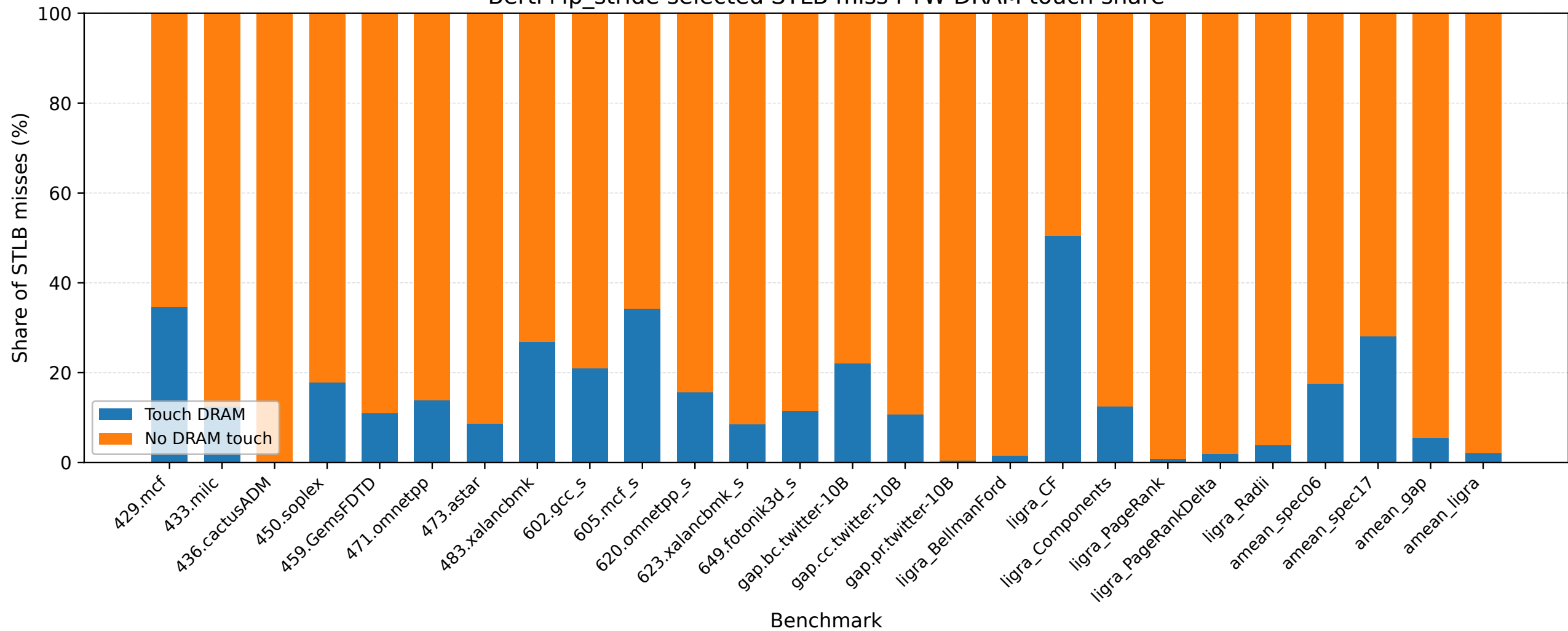
Berti+ip_stride selected STLB miss PTW DRAM touch share
