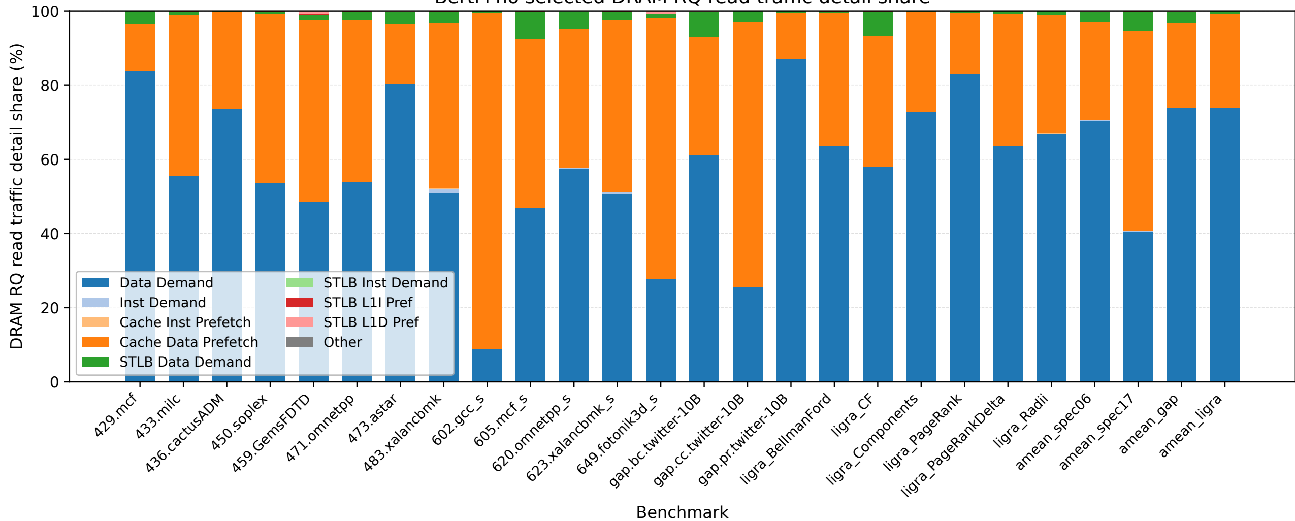
Berti+no selected DRAM RQ read traffic detail share
