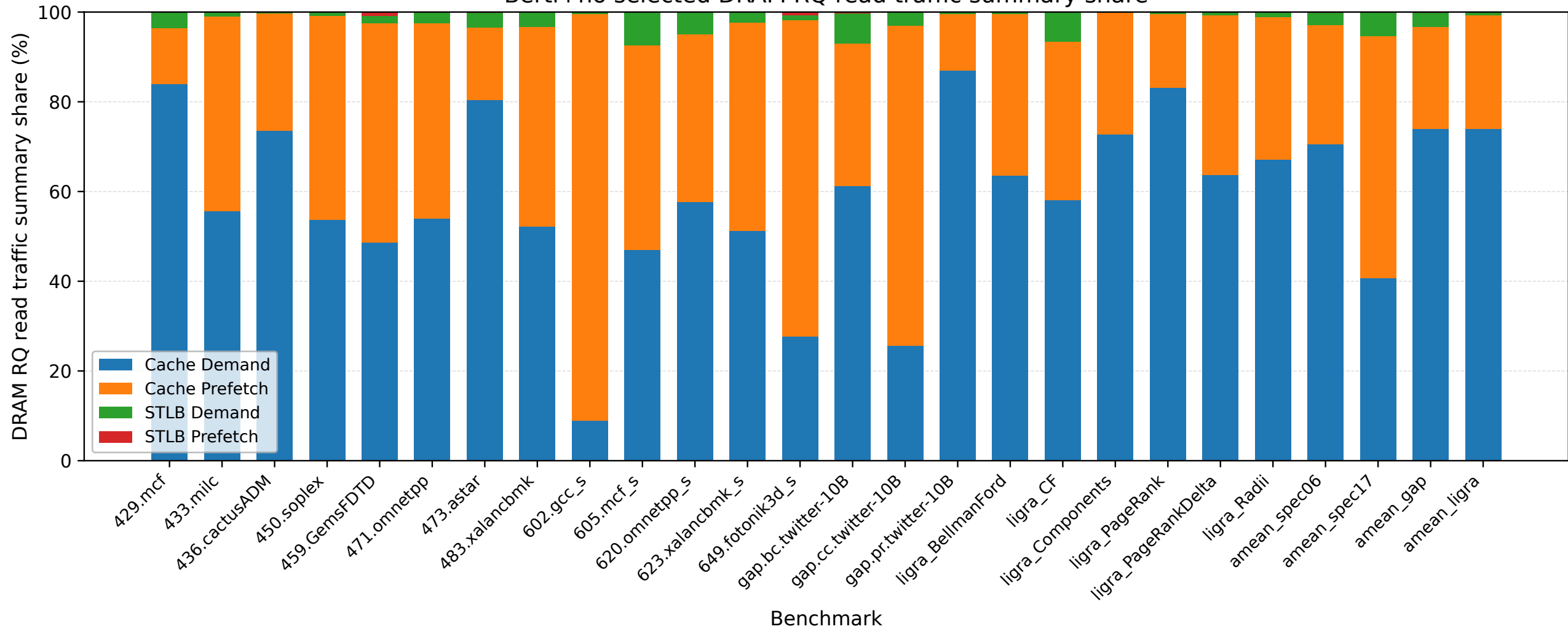
Berti+no selected DRAM RQ read traffic summary share
