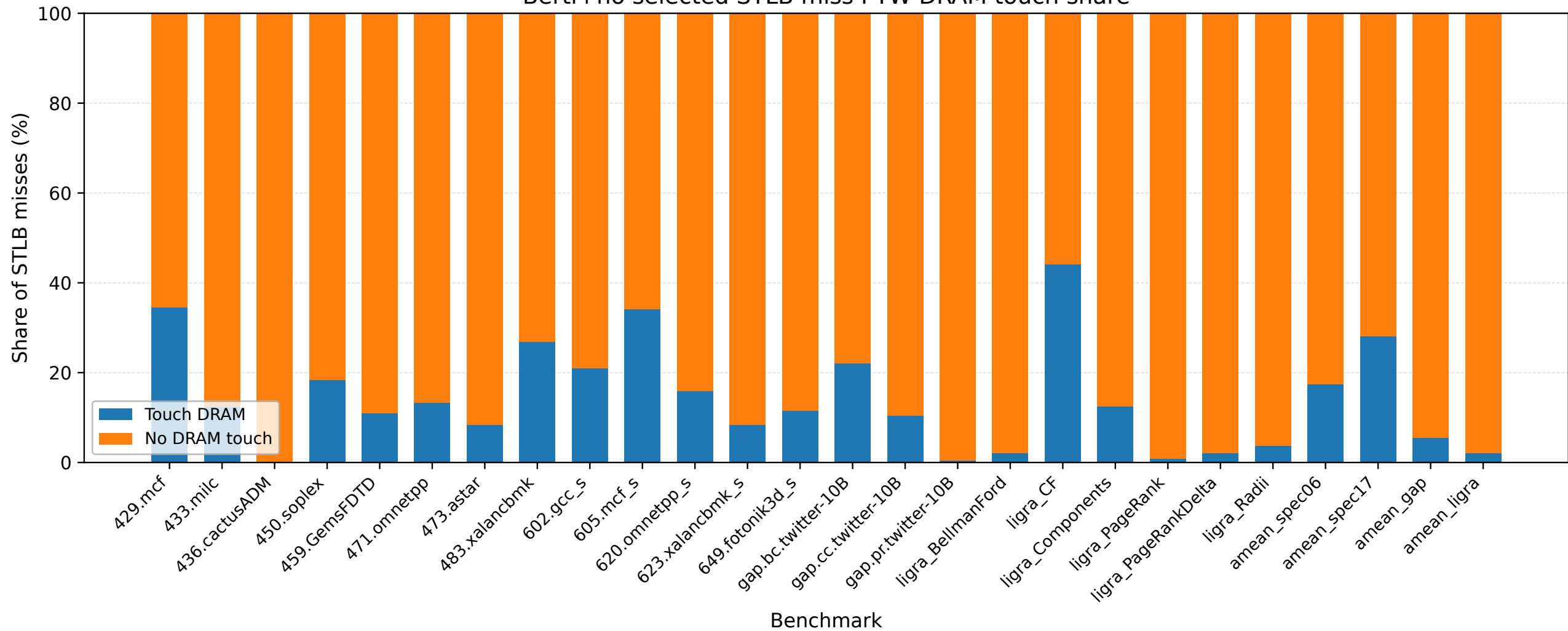
Berti+no selected STLB miss PTW DRAM touch share
