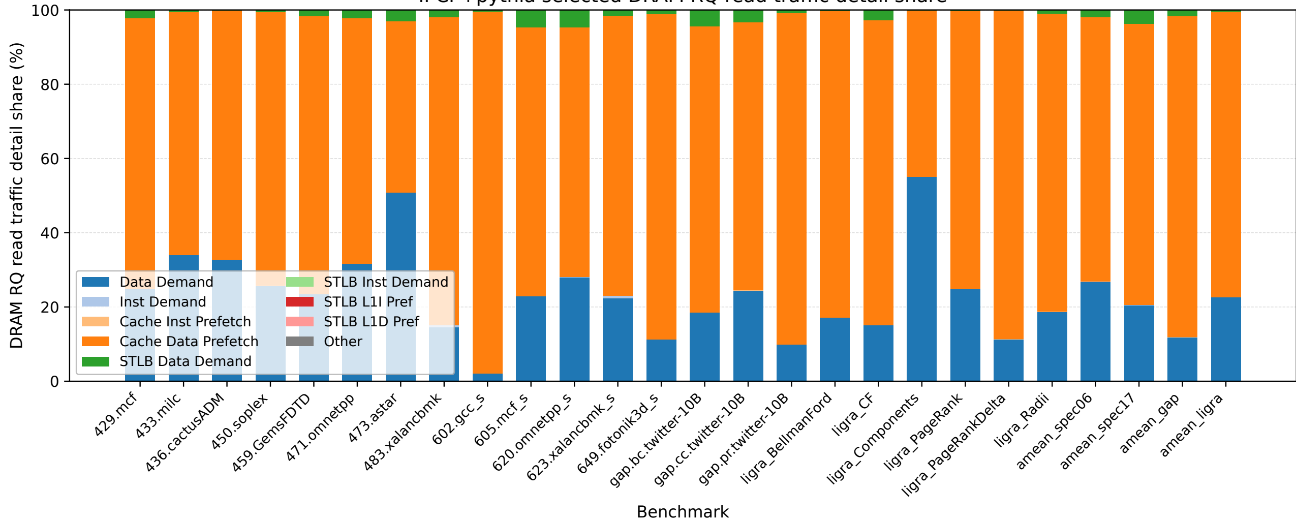
IPCP+pythia selected DRAM RQ read traffic detail share
