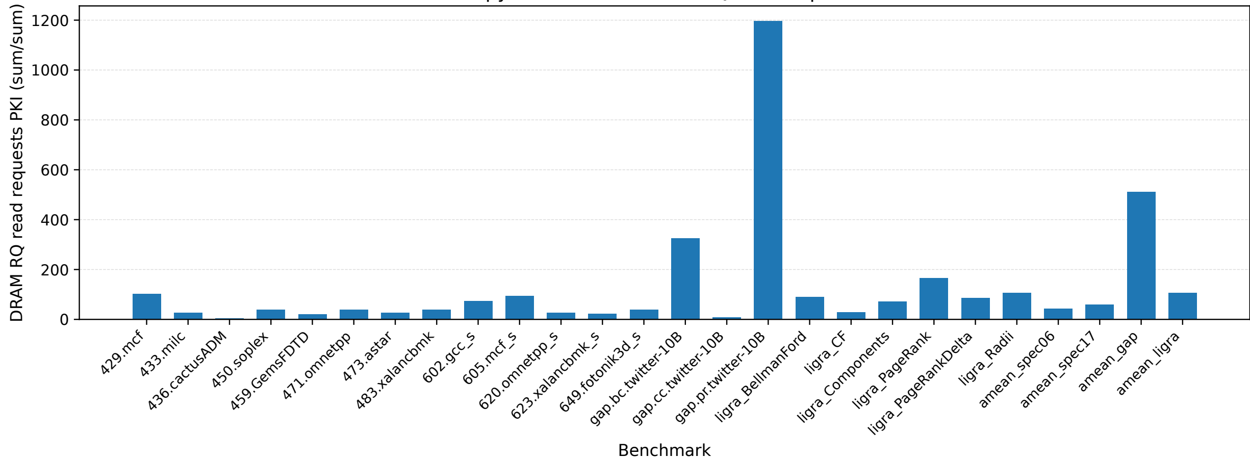
IPCP+pythia selected DRAM RQ read requests PKI
