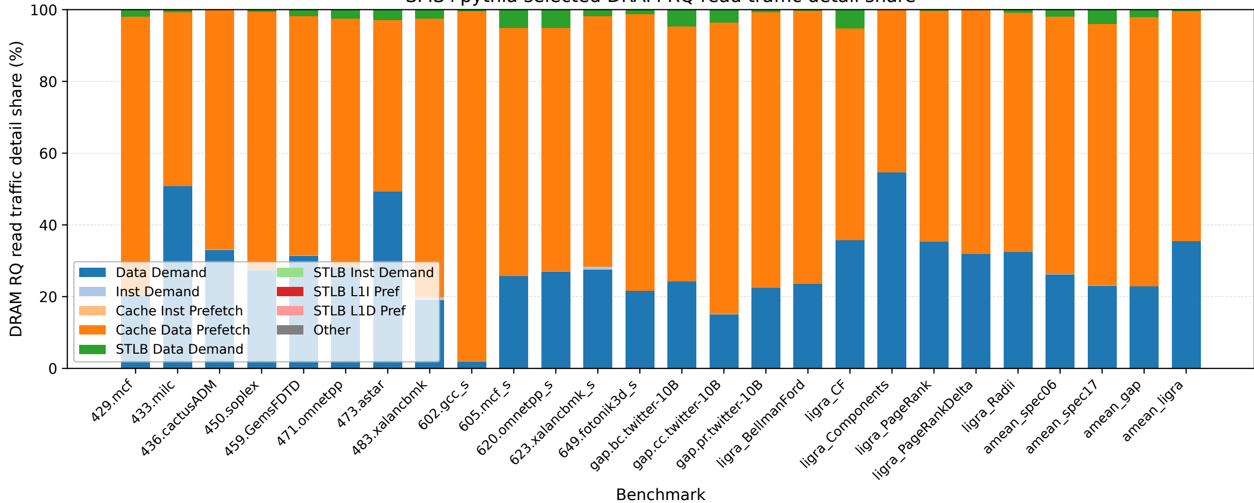
SMS+pythia selected DRAM RQ read traffic detail share
