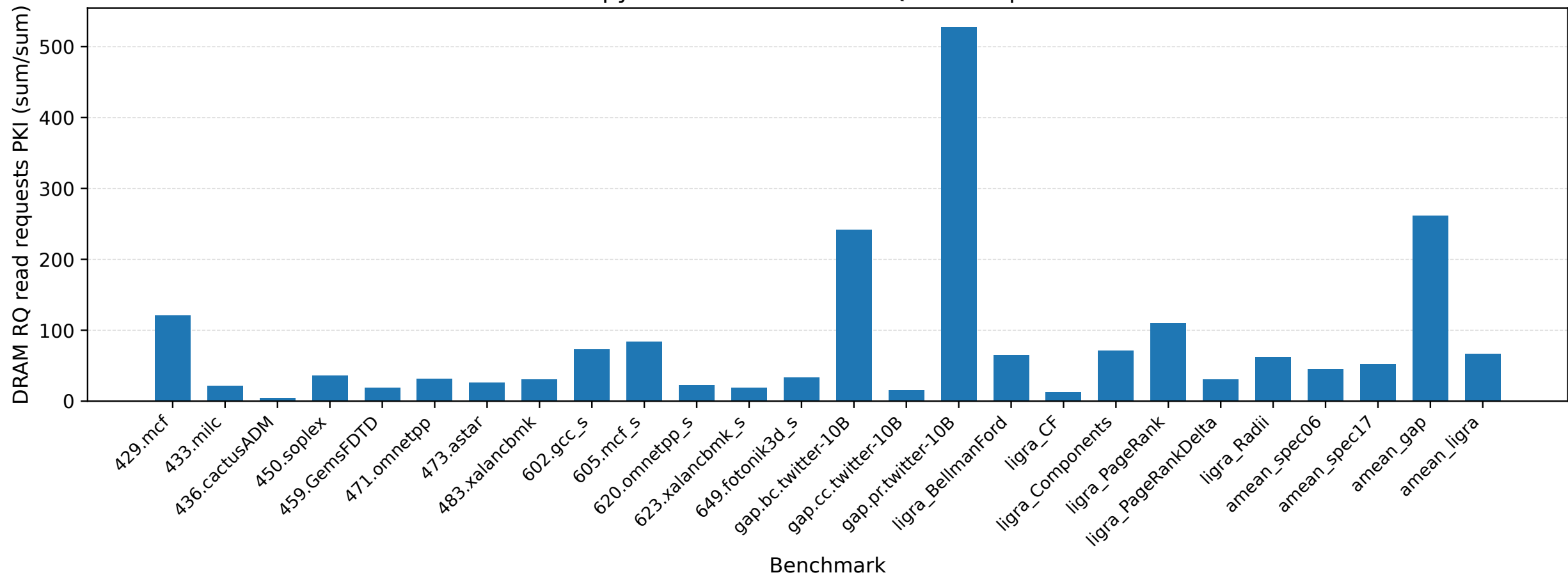
SMS+pythia selected DRAM RQ read requests PKI
