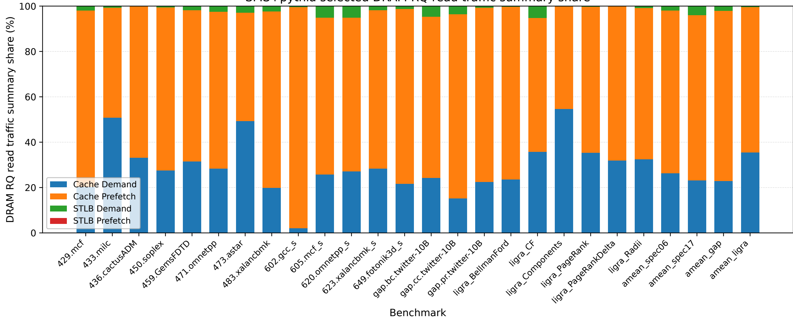
SMS+pythia selected DRAM RQ read traffic summary share
