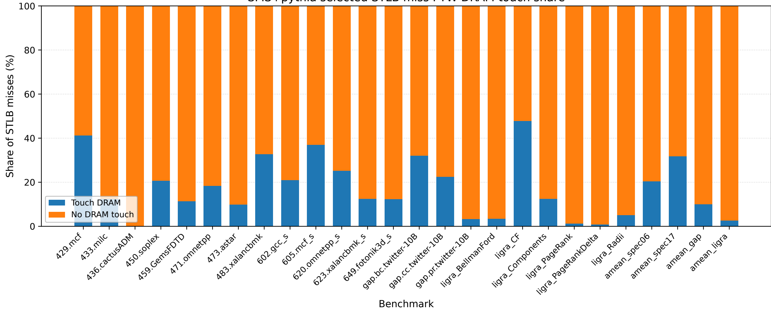
SMS+pythia selected STLB miss PTW DRAM touch share
