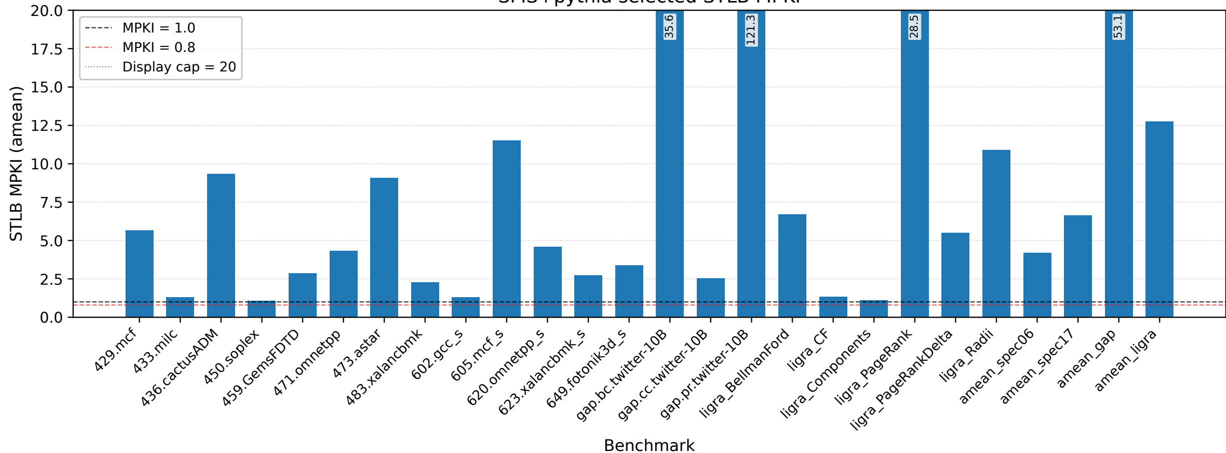
SMS+pythia selected STLB MPKI
