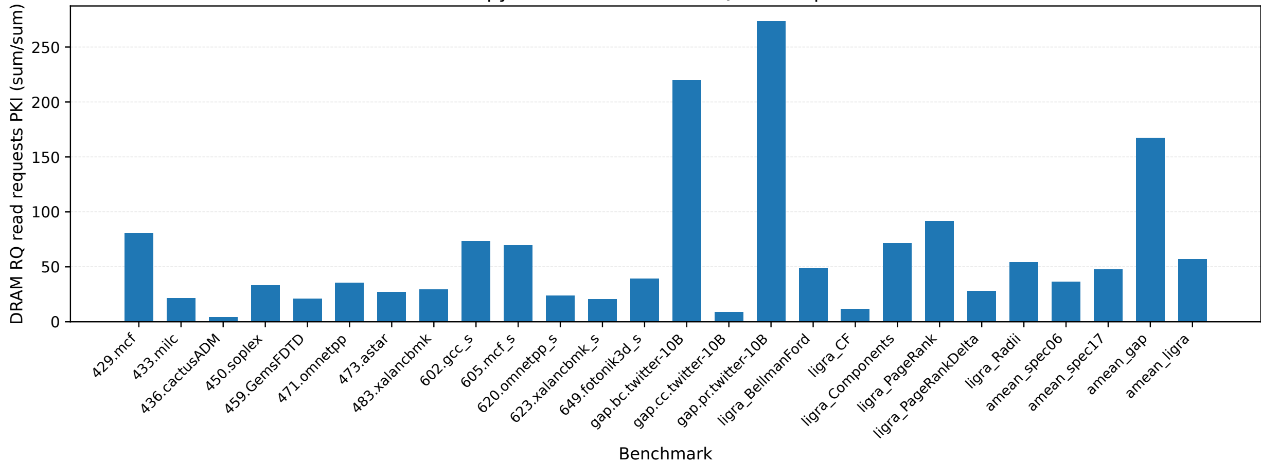
Berti+pythia selected DRAM RQ read requests PKI
