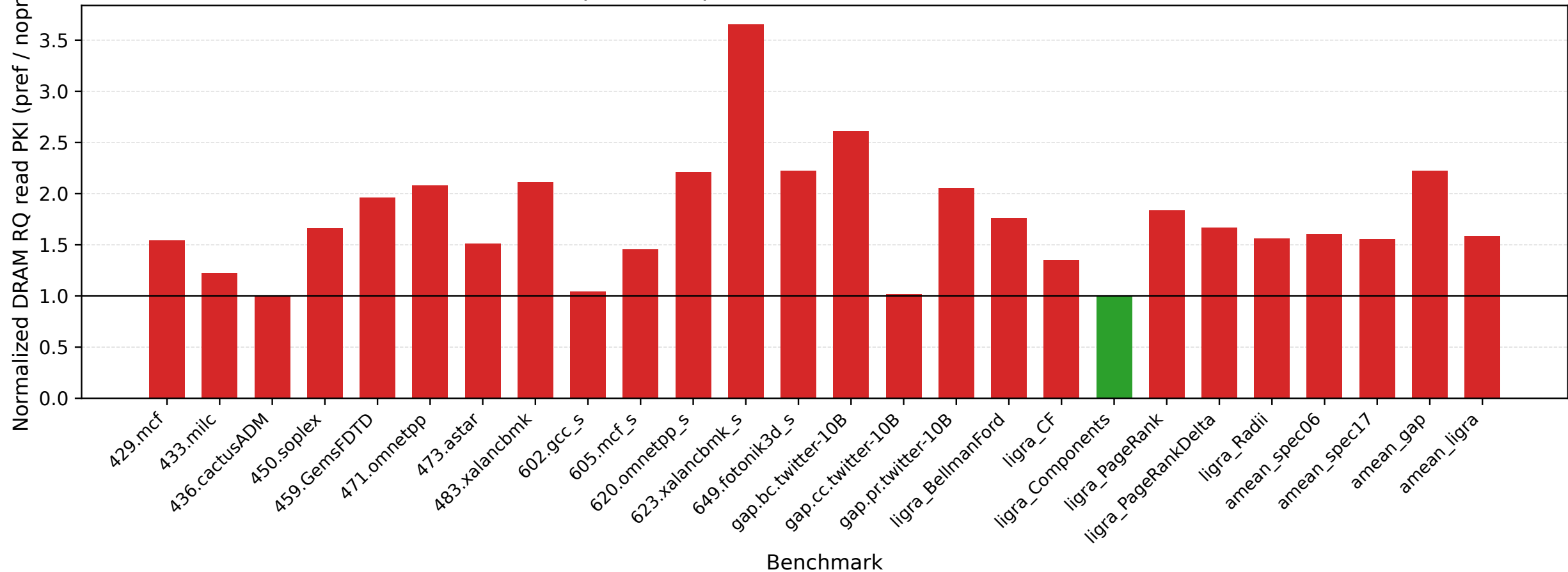
pref vs nopref DRAM RQ read PKI amean
