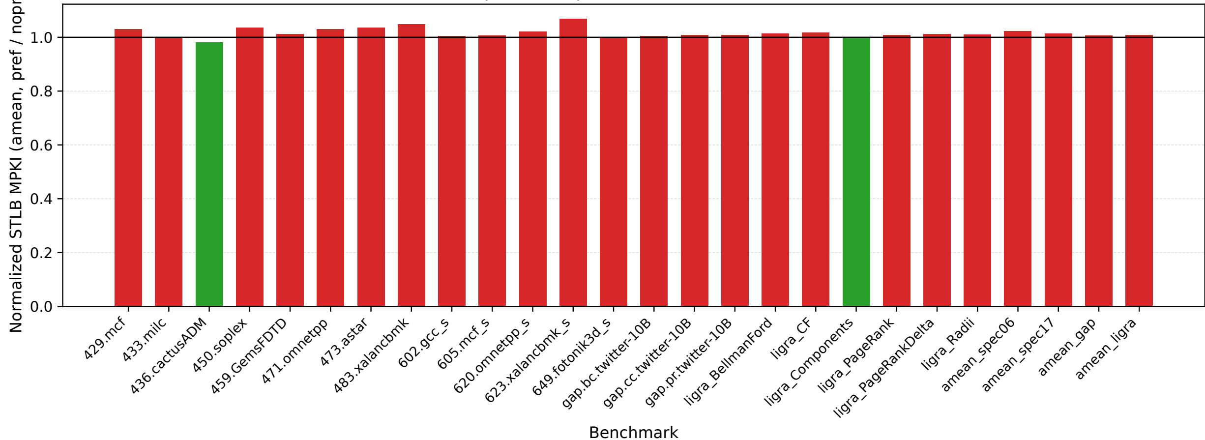
pref vs nopref STLBP MPKI amean
