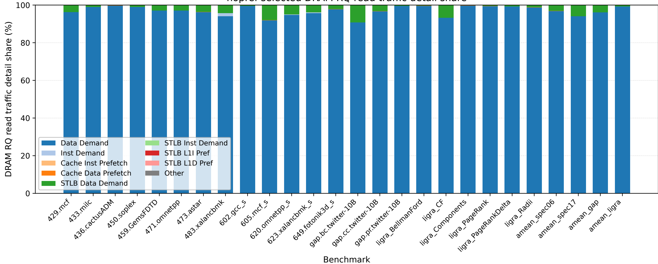
nopref selected DRAM RQ read traffic detail share
