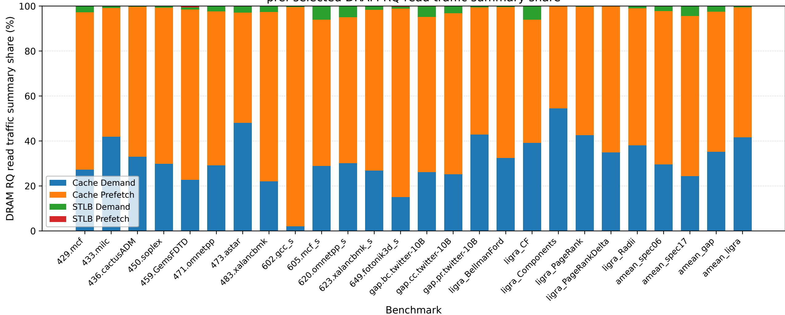
pref selected DRAM RQ read traffic summary share
