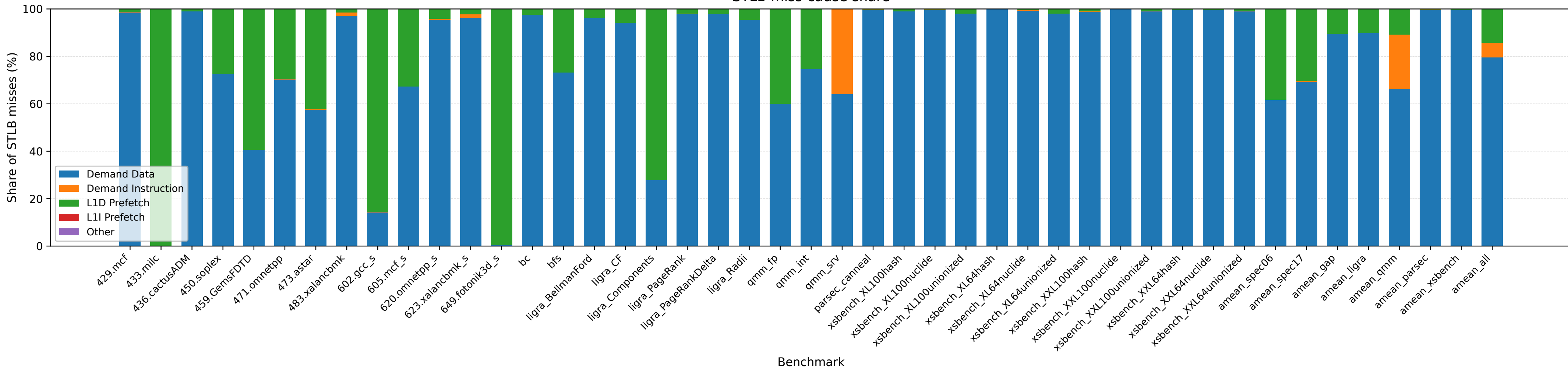
STLB miss-cause share
