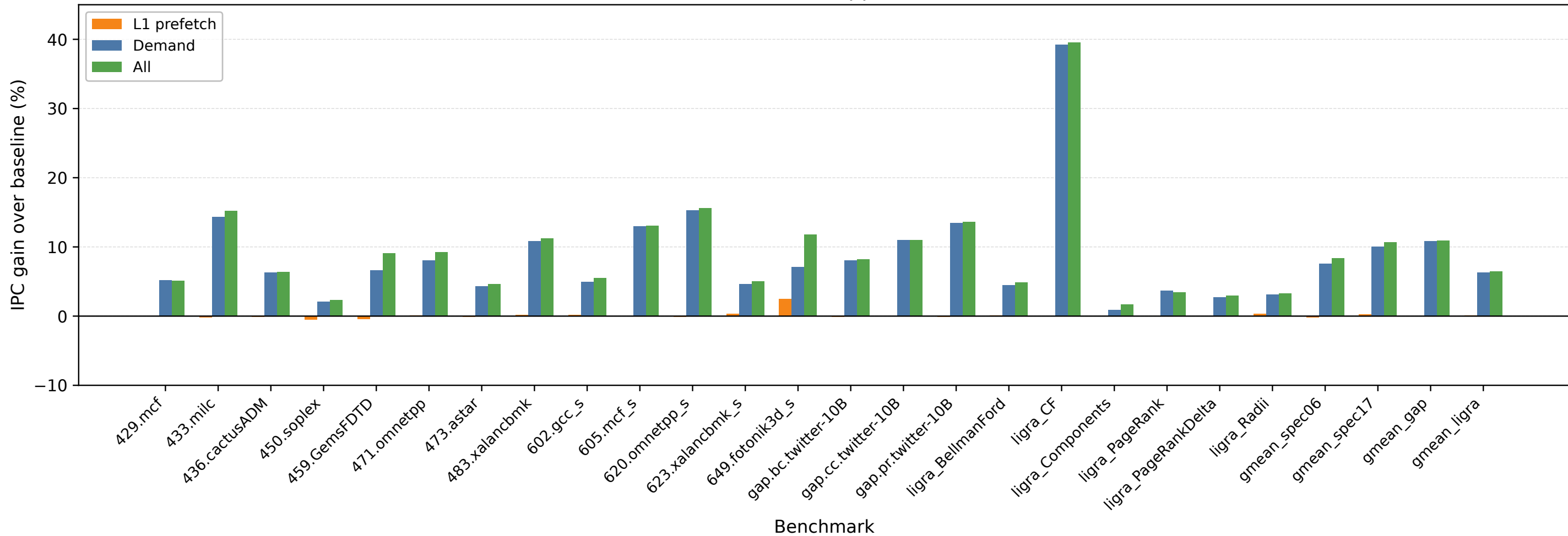
Ideal STLB IPC upper bound
