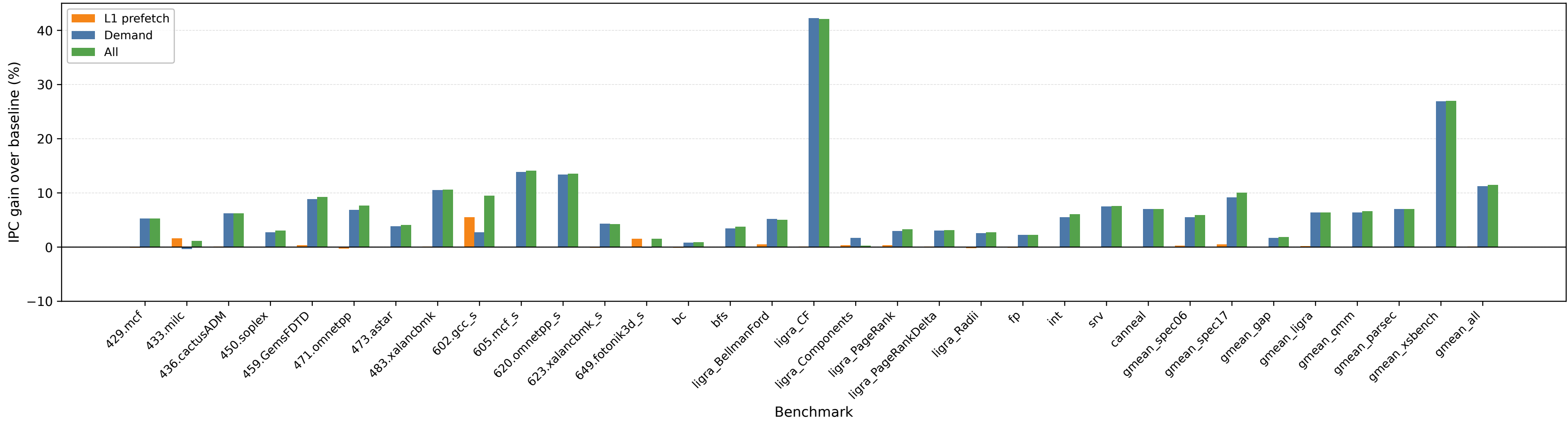
Ideal STLB IPC upper bound
