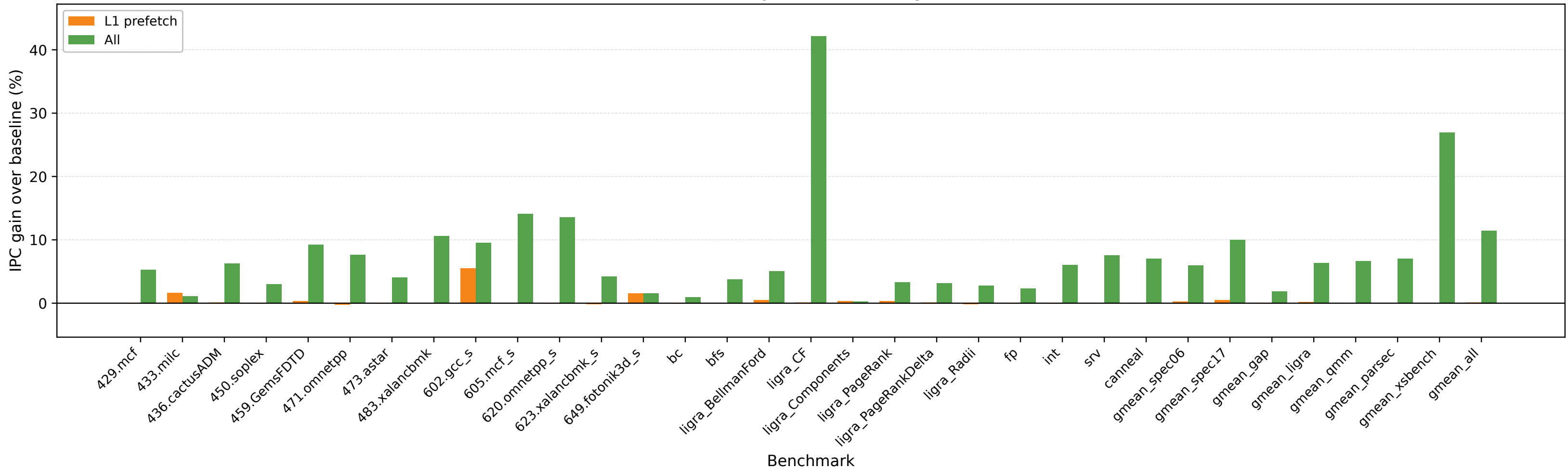
Preliminary ideal STLB IPC gain
