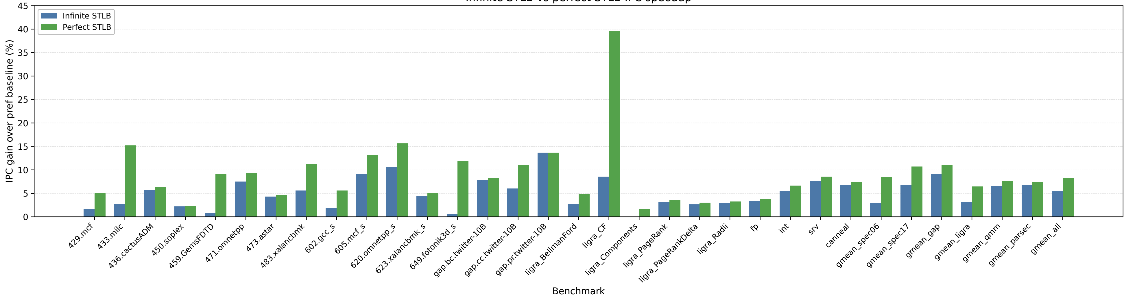
Infinite STLB vs perfect STLB IPC speedup
