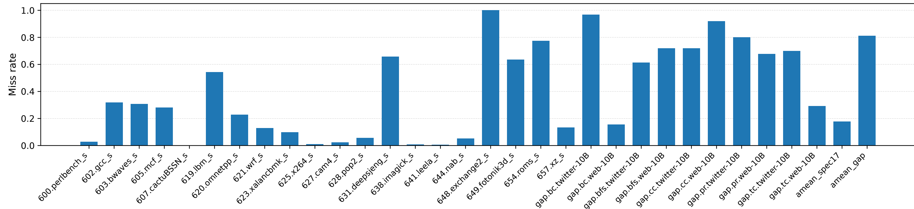
STLB total miss rate
