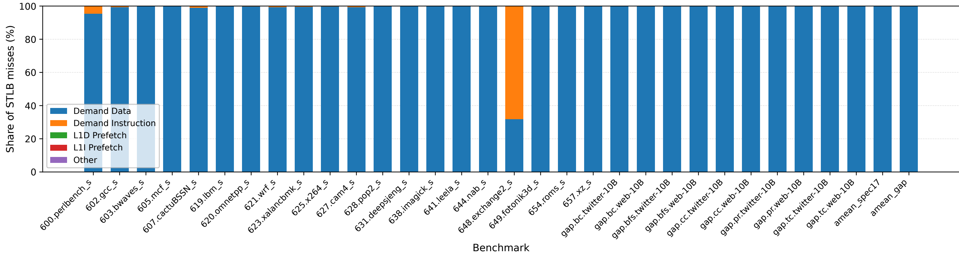
STLB miss-cause share
