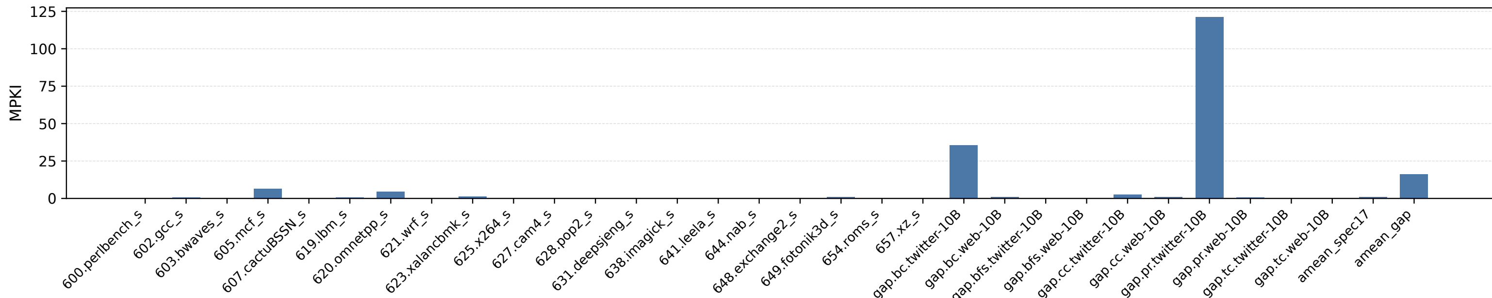
STLB total MPKI
