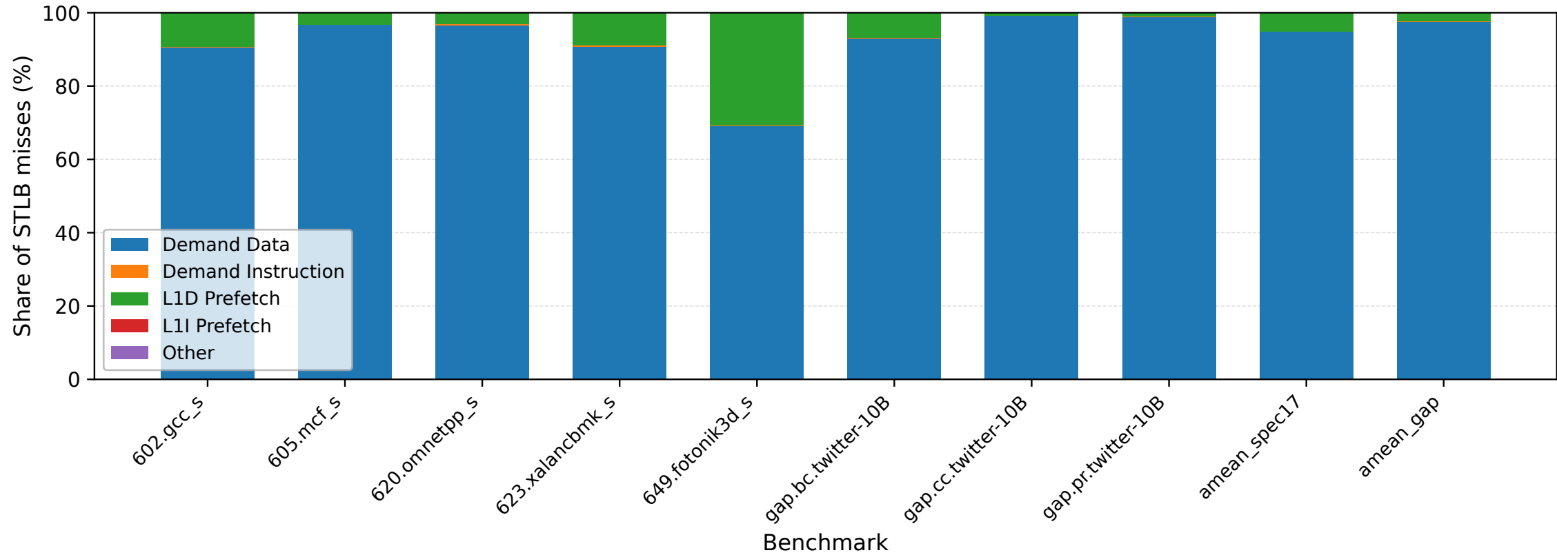
STLB miss-cause share
