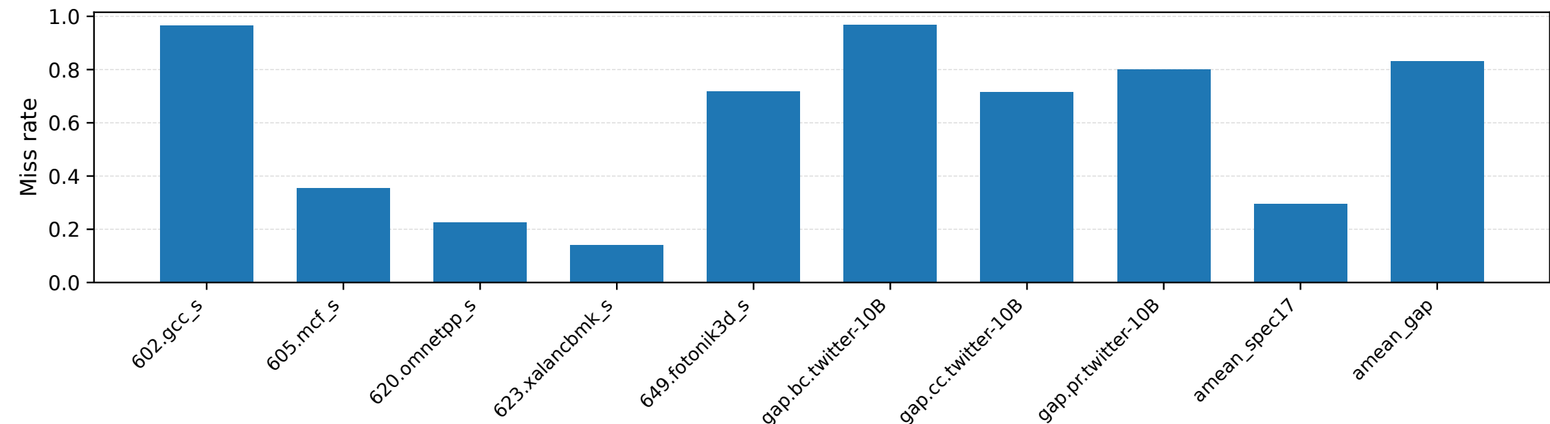
STLB total miss rate
