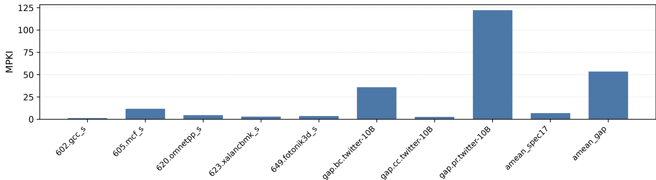
STLB total MPKI
