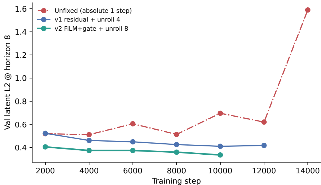
Online validation · lower is better; unfixed diverges
