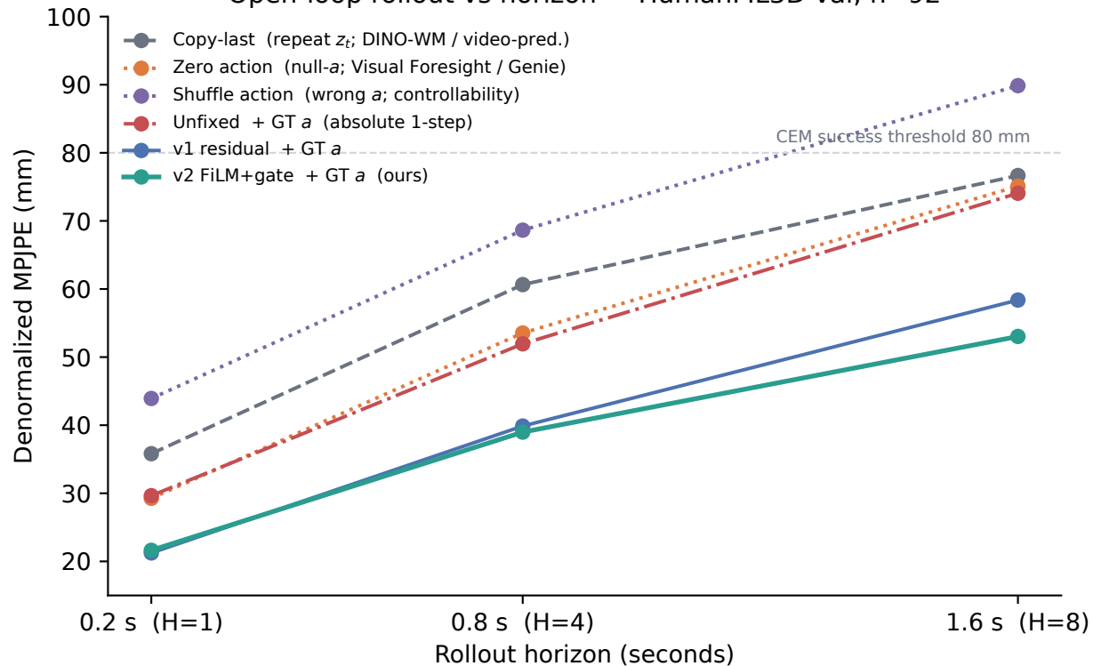
Open-loop rollout vs horizon · HumanML3D val, n=92
