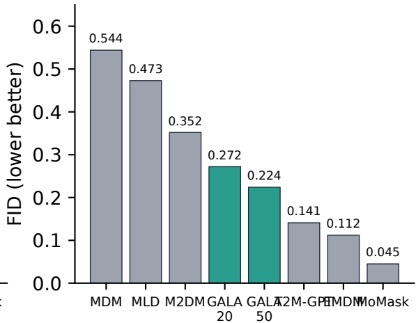
Motion fidelity
