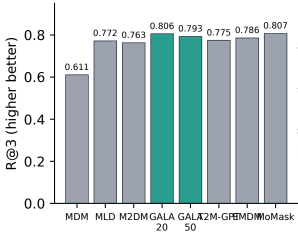
Text alignment
