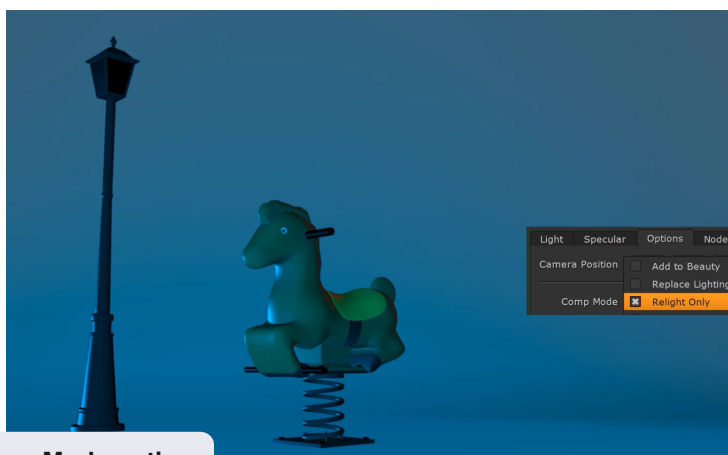
CompMode options
