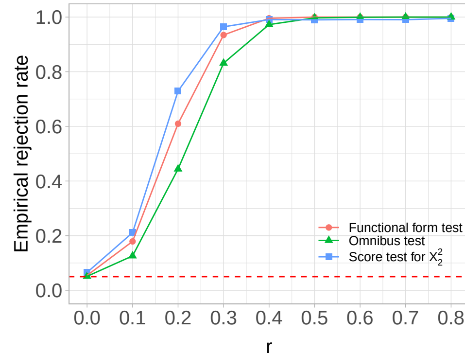
Additional quadratic term, n = 800
