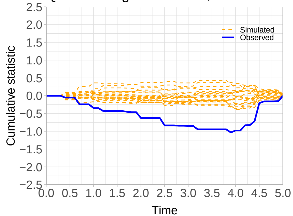
Quadratic log hazard ratio, n = 200
