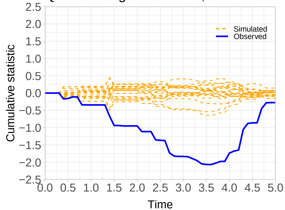
Quadratic log hazard ratio, n = 400
