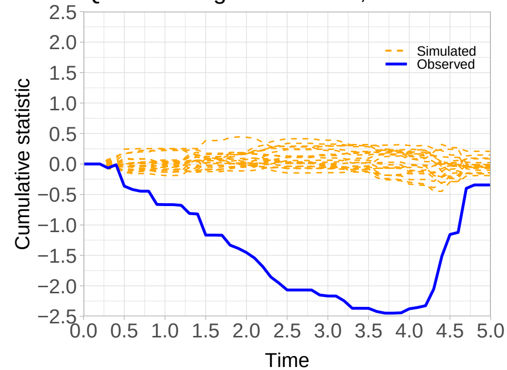
Quadratic log hazard ratio, n = 800
