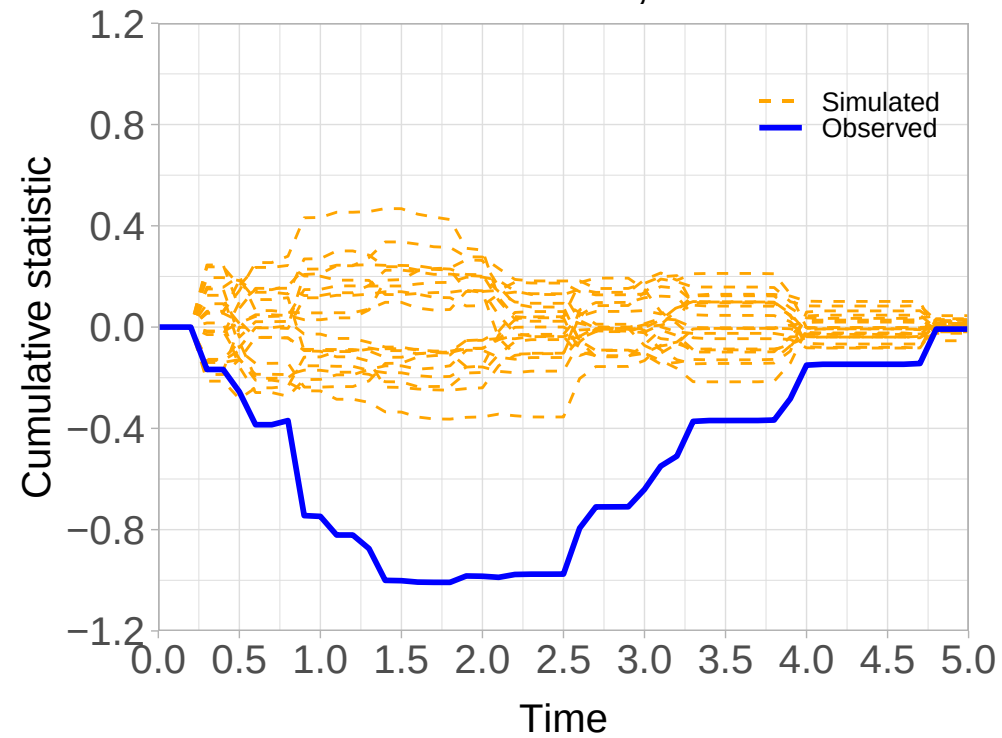
Monotone hazard ratio, n = 400
