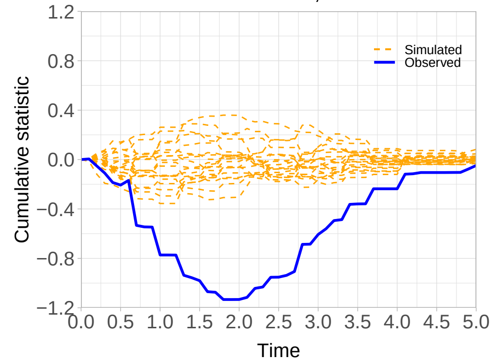
Monotone hazard ratio, n = 800
