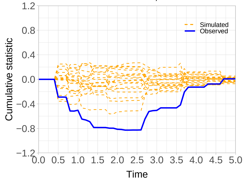
Monotone hazard ratio, n = 200
