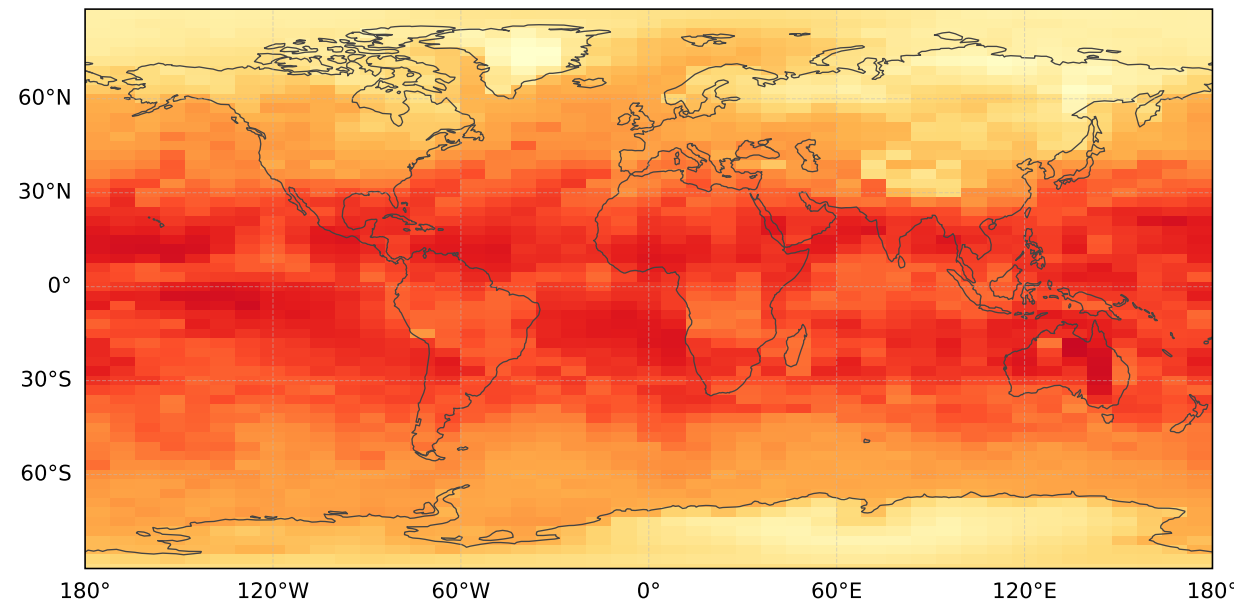
(b) LW OLR (TOA Upward)
