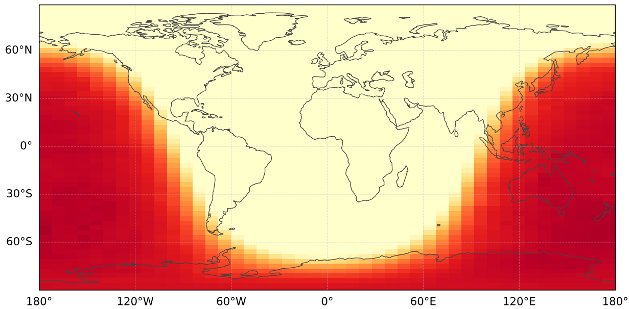
(e) \partial F_{\text{SW}}/\partial \mu_0
