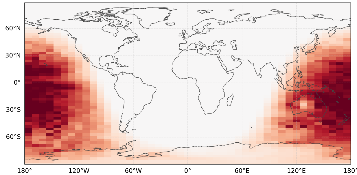
(f) \partial F_{\text{SW}}/\partial T_{\text{sfc}}
