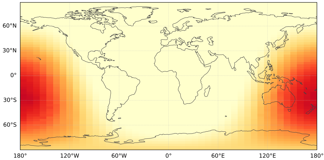
(a) SW Surface Downward Flux
