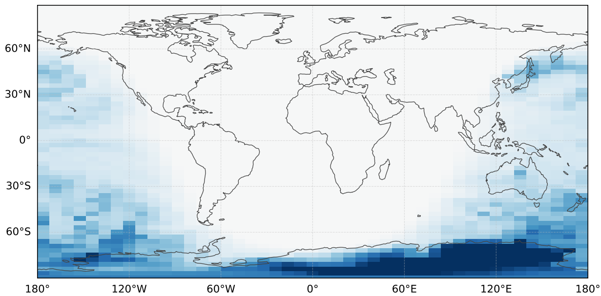
(c) \partial F_{\text{SW}}/\partial q_{\text{sfc}}
