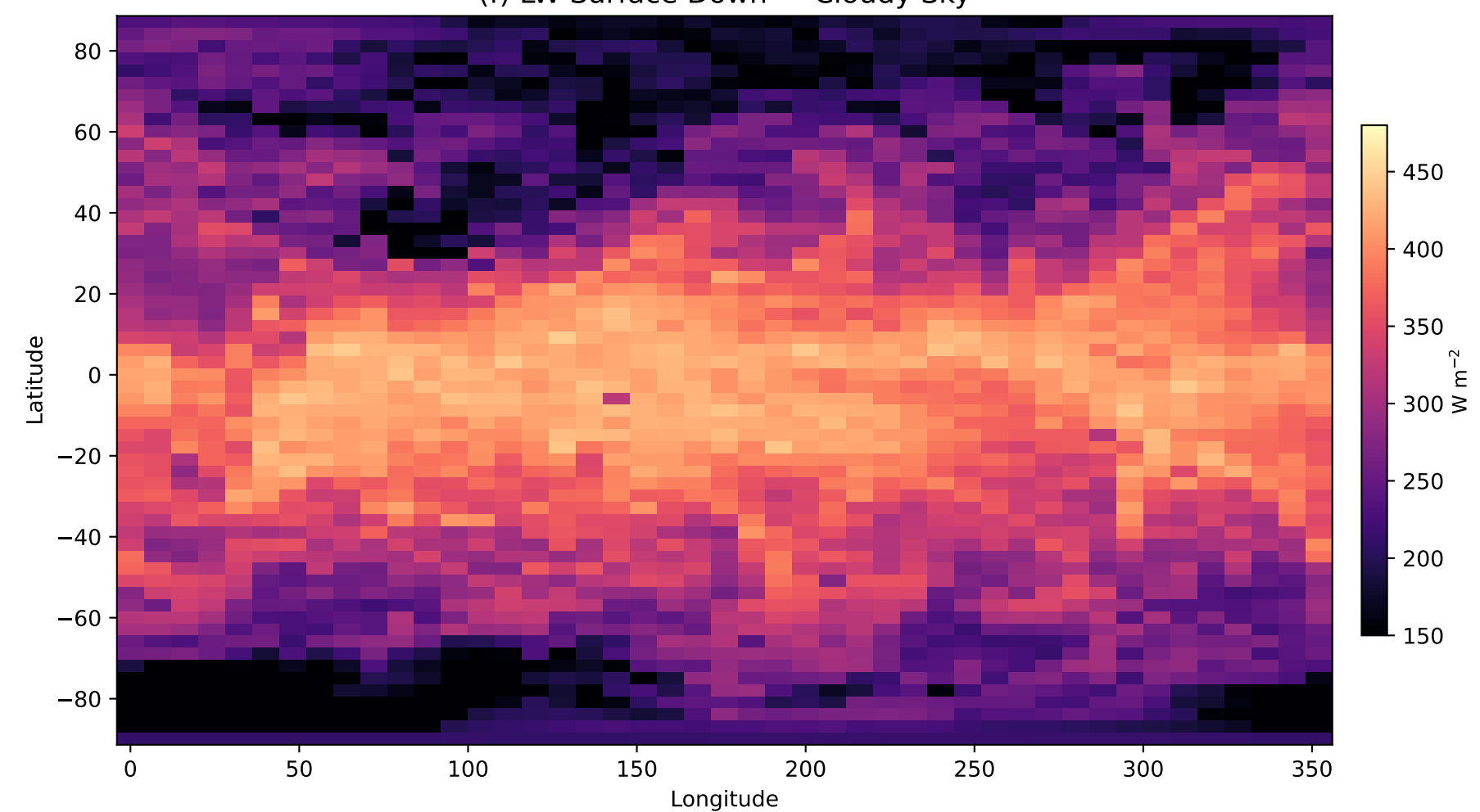
(f) LW Surface Down — Cloudy Sky
