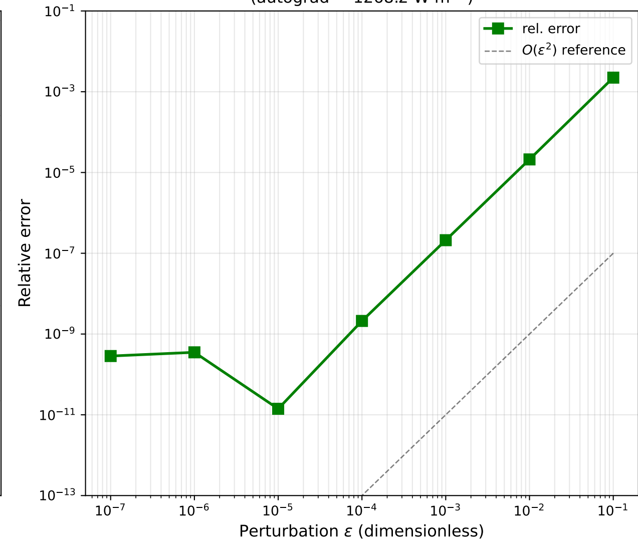
(c) FD Convergence: \partial F_{\text{sfc}}/\partial \mu_0 (autograd = 1268.2 W m ^{-2} )
