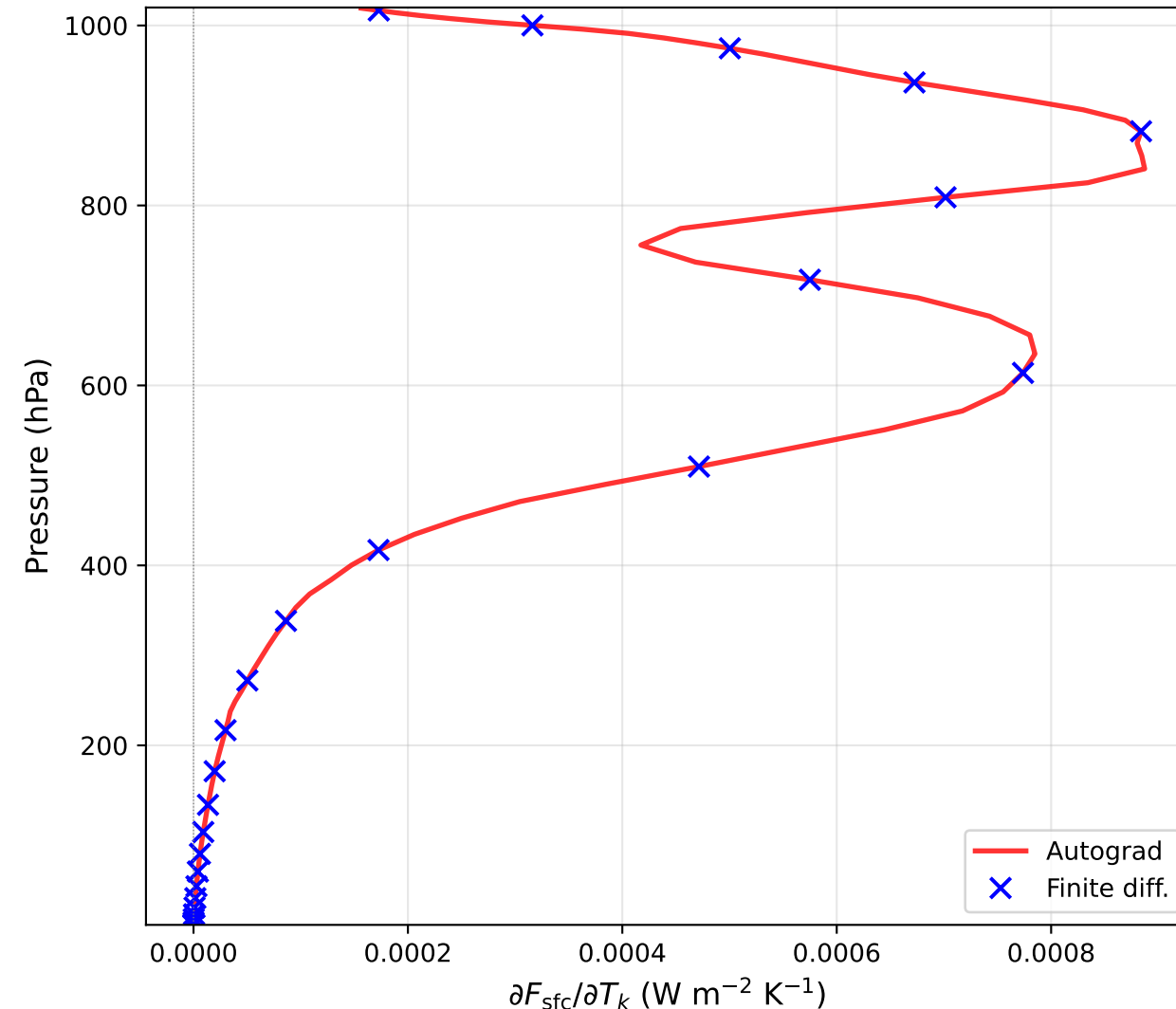
(b) Vertical Gradient Profile \partial F_{\text{sfc}}/\partial T_k at each level
