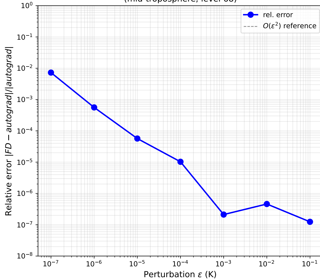
(a) FD Convergence: \partial F_{\text{sfc}}/\partial T_k (mid-troposphere, level 68)
