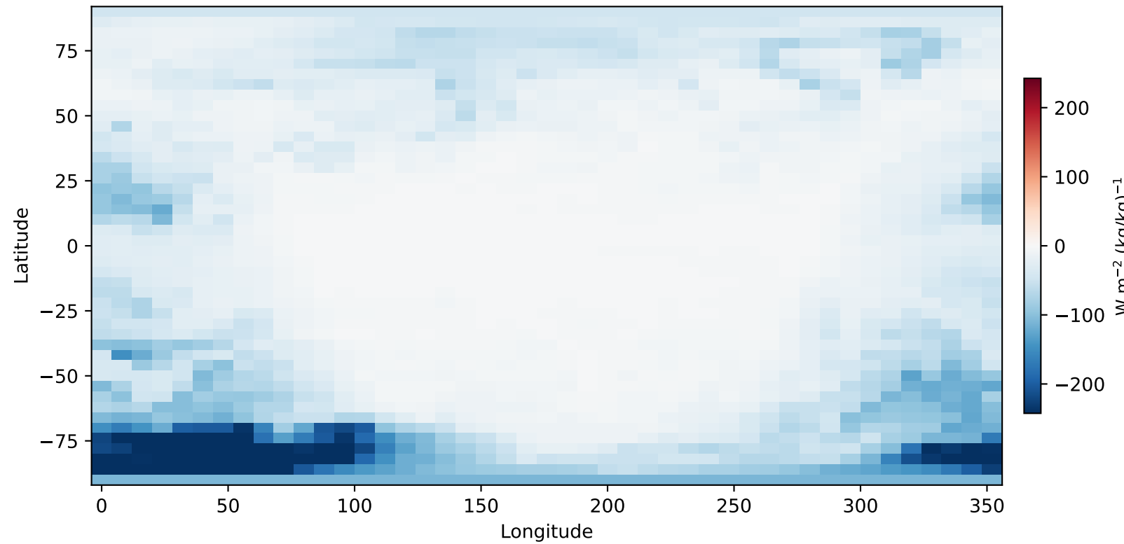
(c) \partial F_{\text{sfc}} / \partial q_{\text{sfc}}
